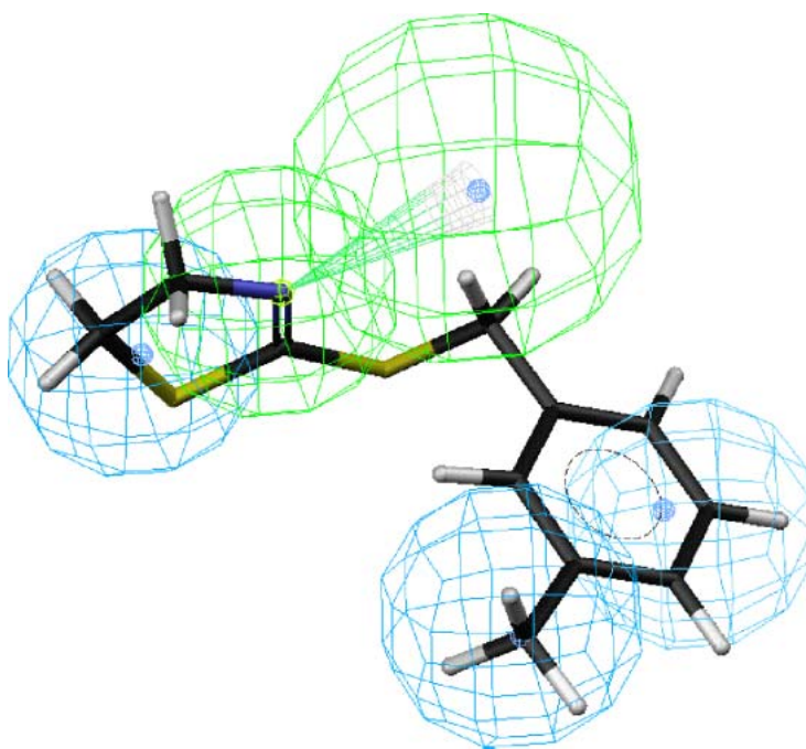
Figure 4. Mapping of 2-(3-methylbenzylamino)-2-thiazoline (43) onto hypothesis 1, which contains an HBAI (green), an HpAr (blue) and two HpAls (blue).
