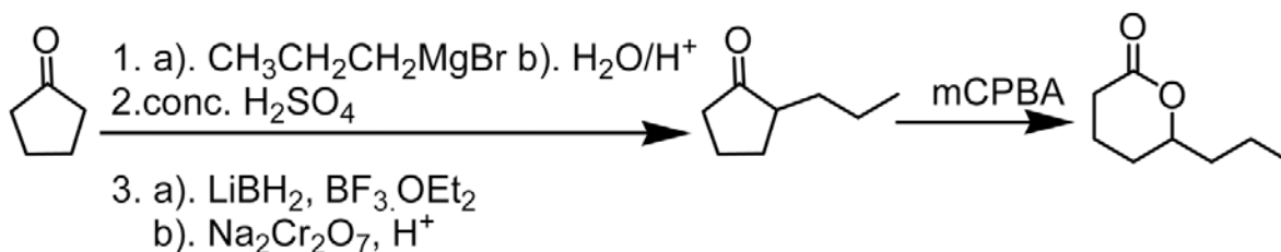
Figure 1. Synthetic scheme for of \delta -octalactone
