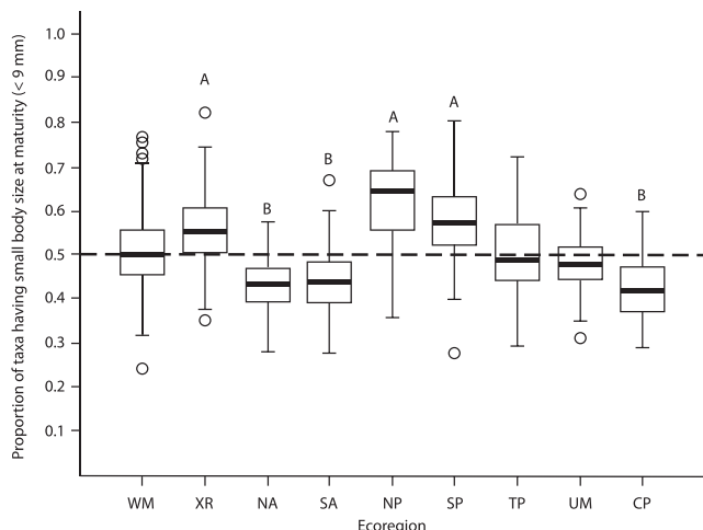
FIG. 2. Example box-and-whisker plot showing the distribution of the proportion of taxa having small body size at maturity (<9 mm) for each ecoregion relative to the average median value (dashed line) for 1257 least-disturbed sites. Boxes represent interquartile range (horizontal line = median), whiskers show values >1.5\times the interquartile range, and open circles indicate outliers. Letters indicate that the trait state was either positively (A) or negatively (B) favored in the associated ecoregion when the interquartile range of the trait state was either above (positively favored) or below (negatively favored) the average median value of all ecoregions (dashed line). We examined similar plots for all trait states to determine which were negatively or positively favored in each ecoregion. WM = Western Mountains, XR = Xeric, NP = Northern Plains, SP = Southern Plains, TP = Temperate Plains, UM = Upper Midwest, NA = Northern Appalachians, SA = Southern Appalachians, CP = Coastal Plain.
