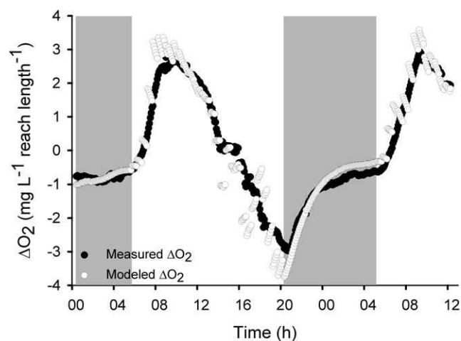
FIG. 5. Change in O_2 ( \Delta O_2 ) between upstream and downstream sampling points of measured and modeled values from Ag North using the fully temperature-corrected model. Shading indicates night time. Each point represents a 10-min period.
