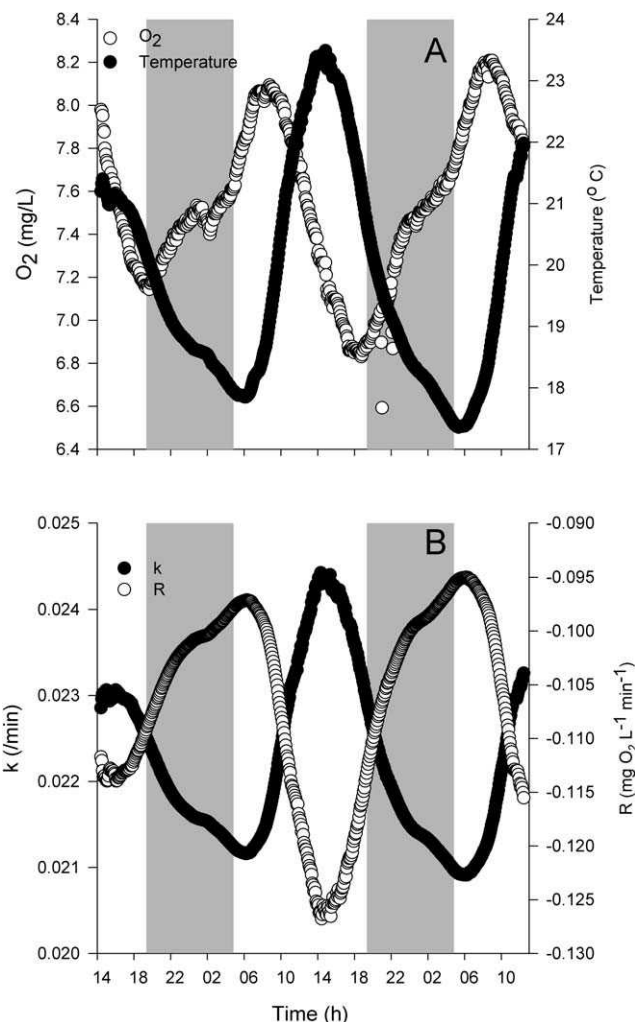
FIG. 7. O_2 and temperature measurements from the downstream O_2 and temperature probe at Natalie's Creek (A) and modeled (fully temperature-corrected model) aeration ( k ) and respiration ( R ) from Natalie's Creek (B). Shading indicates night time. Each point represents a 10-min period.
