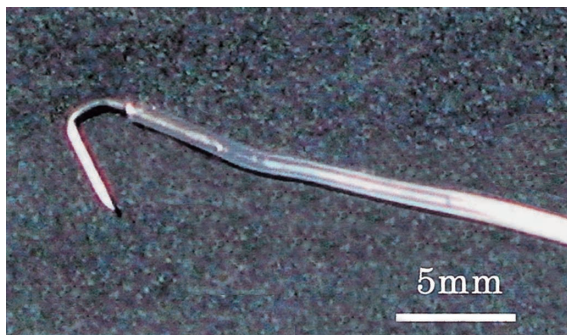
Fig. 1. A photograph showing the cannula using for blood samplings. The top of the cannula is connected with a syringe needle which is bent for insertion to the aortic bulb.
