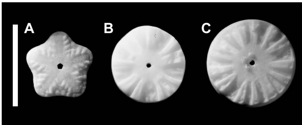
Fig. 3. Articular facets of columnals of Proisocrinus ruberrimus . All from Specimen 3. (A) Columnal from proximal stalk showing its pentagonal outline with five ligamentary fields surrounded by ridges and furrows. (B) Columnal from intermediate stalk. Note circular outline, with radiating ridges and furrows. (C) Columnal from distal stalk. Scale is 5 mm.
