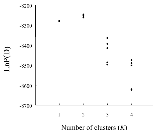
Fig. 1. Plot of estimated logarithms of probability of data [ \text{LnP}(D) ] against number of clusters tested ( K ).
