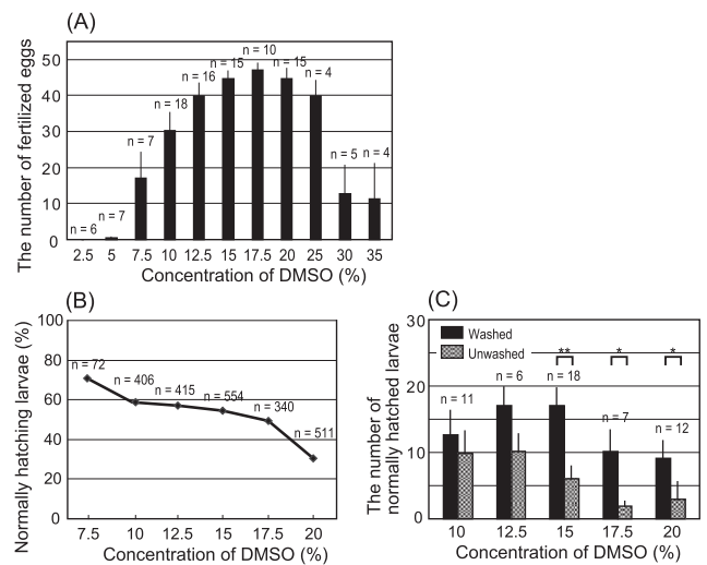
Fig. 2. Optimization of the concentration of DMSO. (A) Fertilization rate obtained using sperm frozen with various concentrations of DMSO. Twenty-microliter sperm suspensions were mixed with 80 µl of ASW containing different concentrations of DMSO (2.5% to 35%). The number of fertilized eggs (as evidenced by the first cleavage) per 50 eggs is plotted on the ordinate (a value of 50 equals 100%). Vertical bars indicate the standard error of the mean. Number of repeated experiments is indicated above each column. A table of the data is presented in Supplemental Table S1 online. (B) The proportion of normal hatched larvae after exposure to different concentrations of DMSO. The proportions of normal hatched larvae are plotted, where the denominator represents the sum of eggs successfully fertilized after insemination with frozen sperm in several experiments, excluding unfertilized eggs. The numerator represents the sum of normally developed larvae in the same experiments. (C) Effect of removal of DMSO after fertilization on normal development. The vertical and horizontal axes indicate the average number of normally hatched larvae among 50 inseminated eggs and the DMSO concentration, respectively. Dark columns indicate the results of removal of DMSO after fertilization, and the gray columns those obtained without DMSO removal. The error bar indicates the amplitude of the standard error of the mean. Removal improved the normal hatching ratio. Double asterisks indicate a p -value of less than 0.01, and a single asterisk indicates a p -value of less than 0.05. Number of repeated experiments is indicated above each column.
