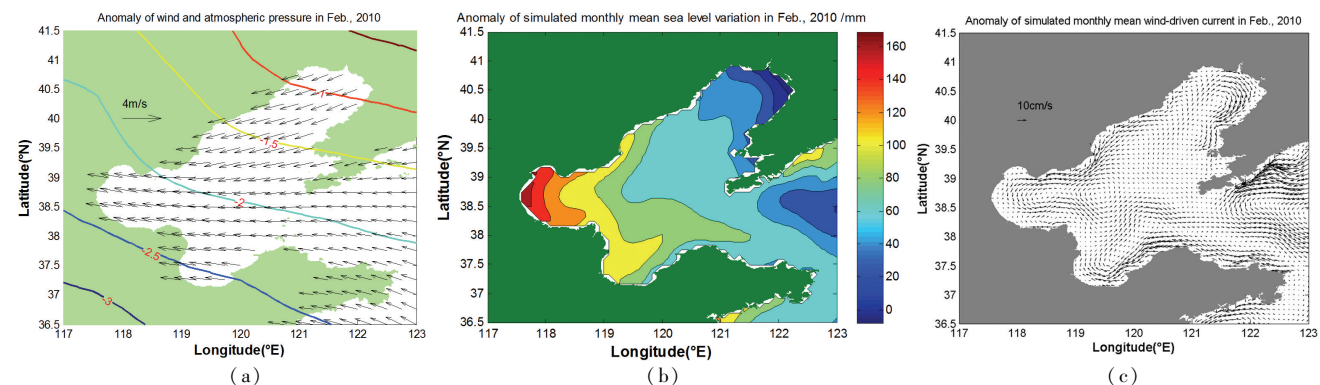
Figure 9. Anomaly of simulated monthly mean sea level variation and wind-driven current, anomaly of wind and pressure in the study area in Feb., 2010
