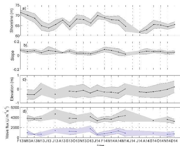
Figure 3. Monthly video estimates of : (a) shoreline location, (b) beach slope, (c) surface elevation, and (d) wave energy flux, cross-shore in grey and longshore in blue. Shaded zones stand for day-to-day dispersion (standard deviation).
