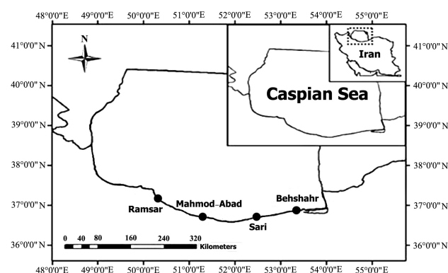
Fig. 1. Location of sampling sites including Behshahr, Sari, Mahmod-Abad and Ramsar in the southern Caspian Sea.
