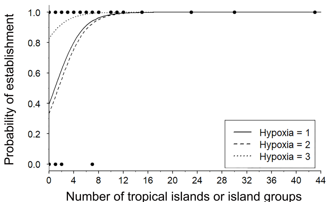
Fig. 2. Probability of establishment of non-native fishes introduced to inland waters of Hawaii and Guam as a function of number of tropical islands/island groups on which a species is established, excluding Hawaii and Guam, and hypoxia tolerance. Logit-scale plots based on mean of fixed plus random family intercept. Hypoxia tolerance score: 1 – intolerant of low dissolved oxygen, 2 – moderately tolerant, 3 – are air-breathers. Closed circles represent number of tropical islands or island groups on which a species is known to be established; many circles represent more than one species.
