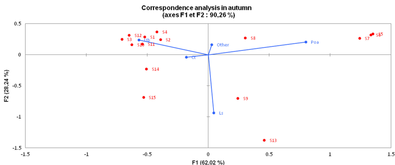
Figure 2. Correspondence analysis of the consumed plant species and individuals of Atlas deer during autumn 2013 in Tazekka National Park. Ct: Cytisus triflorus , Ls: Lavandula stochas , Other: other species, Poa: Poaceae, Ub: Ulex boivini . S i (1 to 15): no. of individuals. Blue circles – plant species, red circles – individuals.
