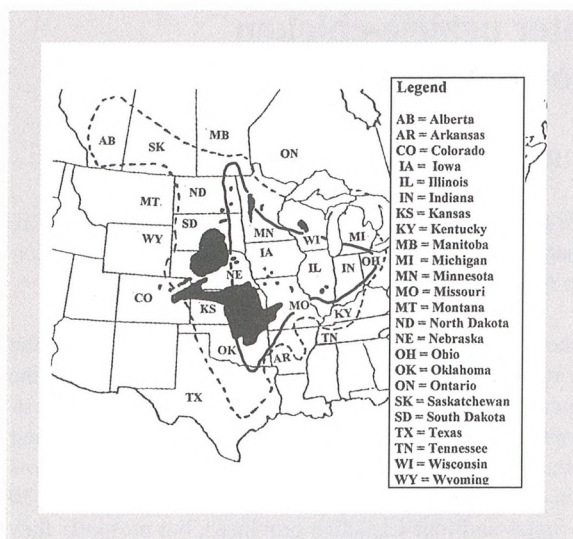
Figure 1. Distribution of the greater prairie-chicken in North America in the past (dashed line; adapted from Schroeder & Robb 1993) and at present (solid areas; adapted from Westemeier & Gough 1999). The solid line delineates the approximate presettlement boundary of the tallgrass portion of the prairie biome (adapted from various sources).
