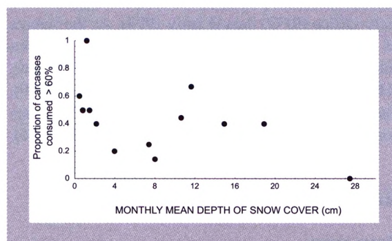
Figure 2. Correlation between proportion of red deer calves consumed (> 60%) by wolves and monthly mean of snow cover depth ( N = 13 ) during the consecutive winters of 1992/93-1994/95 in the Bieszczady Mountains, Poland; ( \tau = -0.42 , P = 0.045 ).
