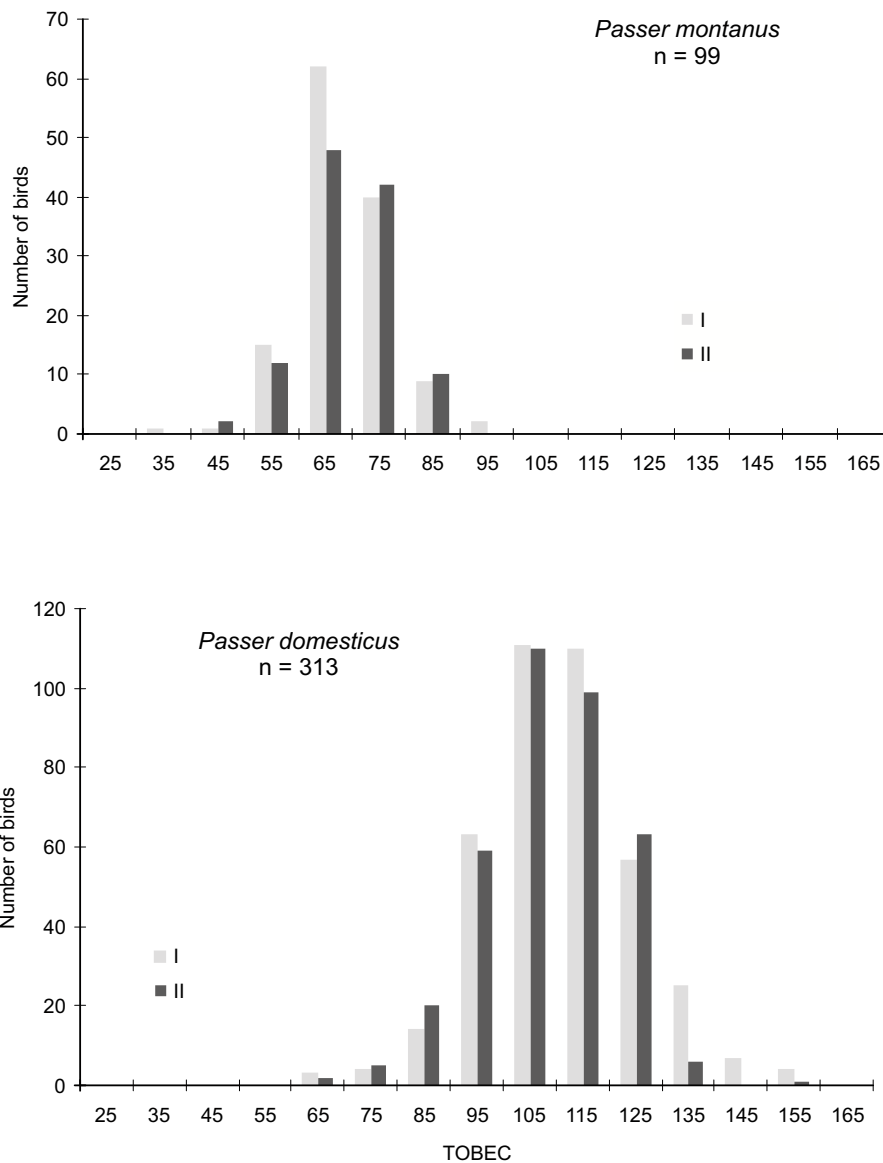
Fig. 1. Distribution of TOBEC readings ( Y_{1j} and Y_{2j} ) obtained in two (I and II) measurements.
