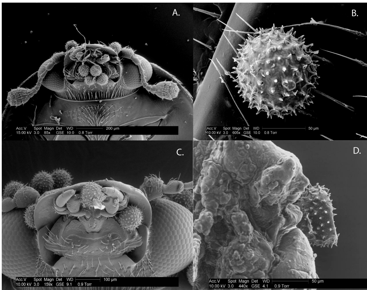
Figure 6. ESEM Micrographs A) Aethina concolor with Gossypium tomentosum pollen clustered on the head. B) Gossypium tomentosum pollen in the setae of a nitiulid beetle, Aethina concolor . C) Aethina concolor with G. tomentosum pollen in its mandibles. D) Gossypium tomentosum pollen inside the dissected GI tract of a nitiulid beetle.
