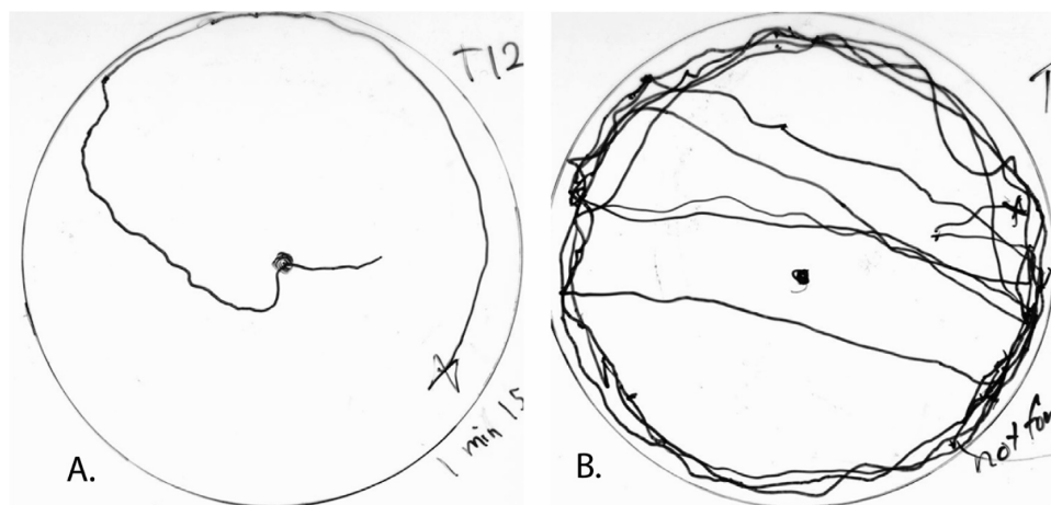
Figure 7. A sample of tracing patterns on the transparencies from the tracing experiments with Aethina concolor beetles. A. Beetle tracing pattern when treatment source had a color component. B. Beetle tracing pattern when treatment source had no color component.
