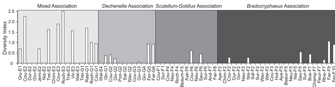
Fig. 5. Diversity (Shannon-Weaver index) of the 67 trilobites samples from the Middle and Upper Devonian of the Ardenne Massif and Boulonnais (North France, Belgium) for four delineated associations (see Figs. 2, 3 for abbreviations).
