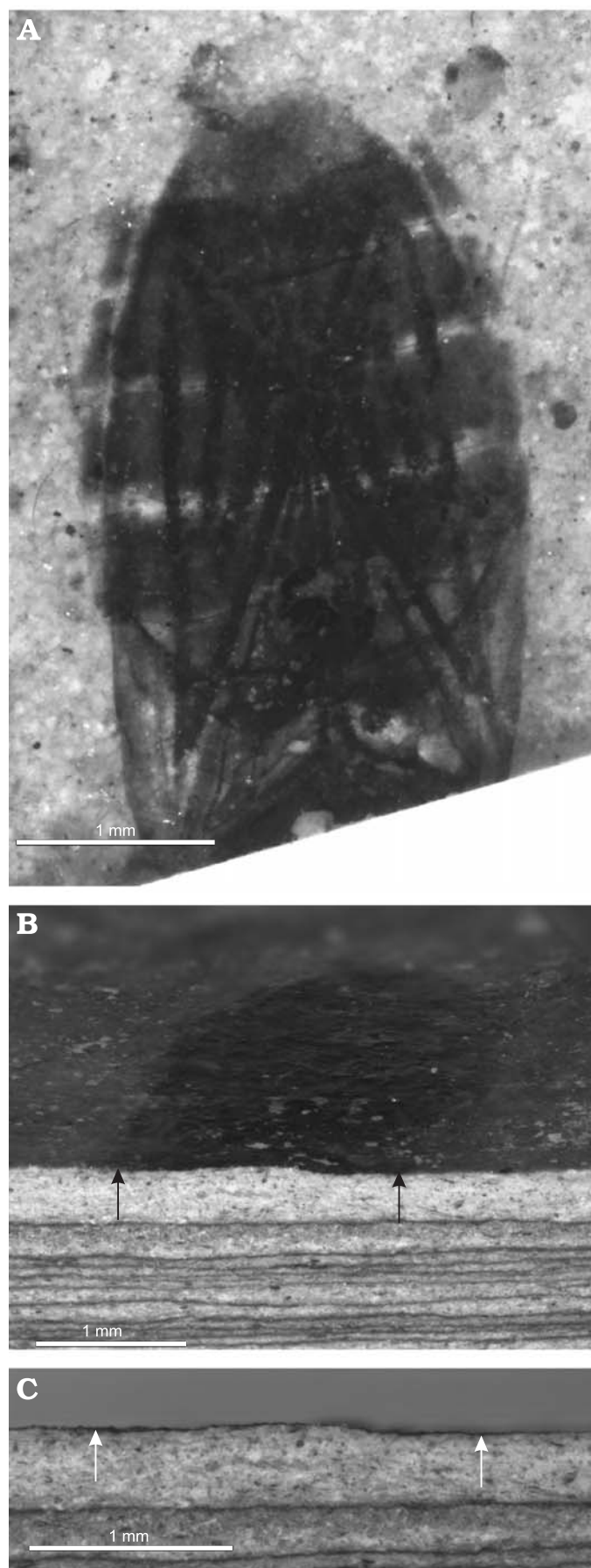
Fig. 12. A varve surface in shale (USNM 560104) from the Coal Creek member of the Kishenehn Formation, Eocene, Montana, USA, in which the fossilized microbial mat contains a water boatman (Hemiptera: Corixidae). A. A photograph of the fossil corixid immersed in ethanol. B. An oblique view of a cross-section of the dry specimen. Note the varves of widely variable thickness. The corixid (between the arrows) is on the surface of the rhythmite within the microbial mat. C. Cross-section showing the only slightly thickened mat at the site of the corixid fossil (arrows).
