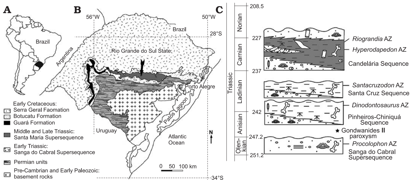
Fig. 1. A. Map of South America with the state of Rio Grande do Sul shaded. B. Location of the Agudo municipality (arrow) in the state of Rio Grande do Sul, where Middle and Upper Triassic rocks crop out. C. Sequence stratigraphy of Brazilian rocks containing Triassic vertebrates, with the Hyperodapedon Assemblage Zone highlighted (modified from Horn et al. 2014).
