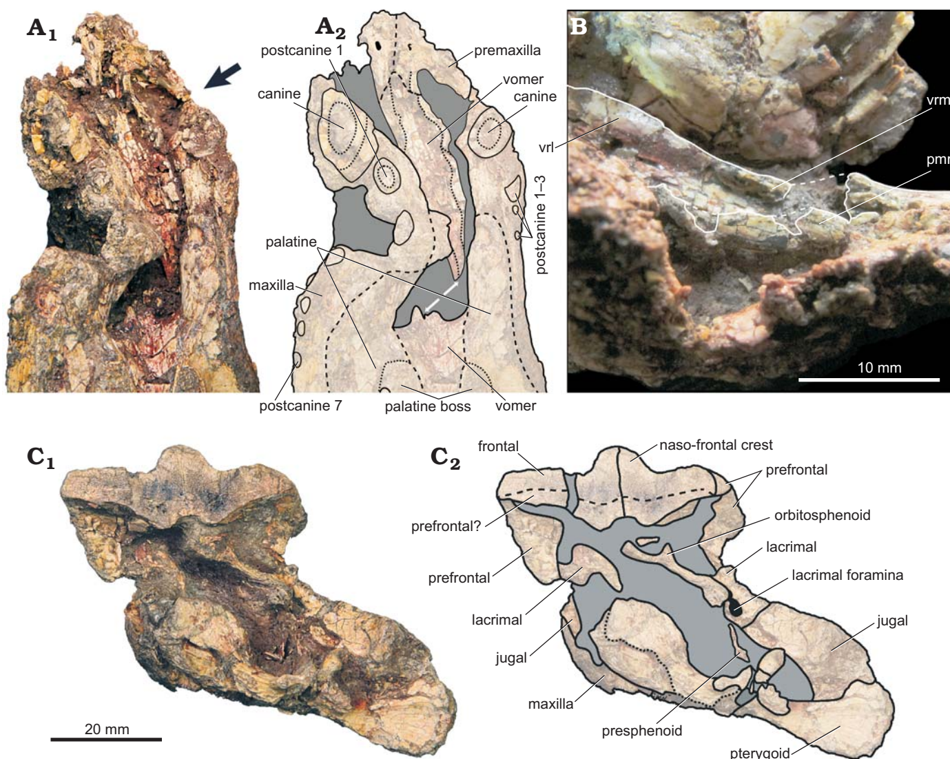
Fig. 5. Burnetiamorpha gen. et sp. indet. (BP/1/7098) from Springfontein, Beaufort West district, South Africa; upper Poortjie Member, Pristerognathus AZ, latest Capitanian. A. Anterior palate in ventral view, black arrow shows direction of view in B; white arrows show lateral displacement of interchoanal portion of the vomers. B. Interchoanal portion of vomers in right ventral view ( B ), showing the continuation of the downturned edges of the vomer extending anteriorly onto the premaxilla; pmr, ventral ridge of premaxilla at anterior margin of choana; vrl, ventral ridge of vomer laterally flared; vrm, ventral ridge of vomer medially folded. C. Specimen in posterior view. Photographs (A 1 , C 1 ) and explanatory drawings (A 2 , C 2 ).
