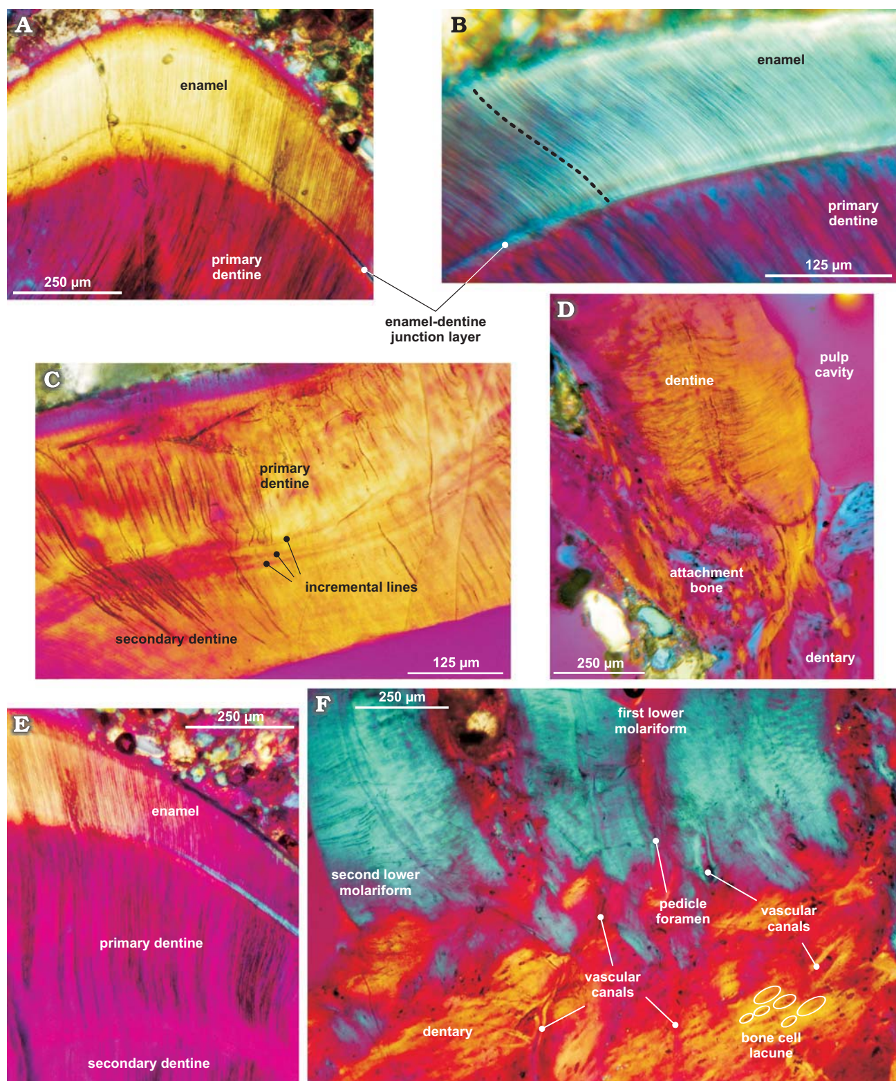
Fig. 2. The procolophonid Soturnia caliodon Cisneros and Schultz, 2003, UFRGS PV1112T, from the Norian (Upper Triassic) Caturrita Formation of Rio Grande do Sul, Brazil. A. Enamel and primary dentine from the apical region of m2. B. Enamel and primary dentine from the region between the apex and the cervix of m2. The slightly sigmoid curvature of the crystallites is highlighted by a dashed line. C. Primary and secondary dentine in the anterior portion of the cervical region of m2. Note the irregular primary dentinal tubules compared to those in the apical region (A and E). D. Attachment bone in the posterior region of the base of m2. E. Primary dentine in the apical region of m2. F. Tooth implantation in m1 and part of m2. Attachment bone, characterized by globular or irregular bone cell lacunae, is predominant in the reddish areas of the photograph. Dentine is shown in blue, note some small amounts of pedicle dentine within the dentary bone. Dentary bone tissue, represented in yellow and orange, showing predominance of elongated and anteroposteriorly directed bone cell lacunae. The apex is placed to the left in B and C. All photographs taken using polarized light.
