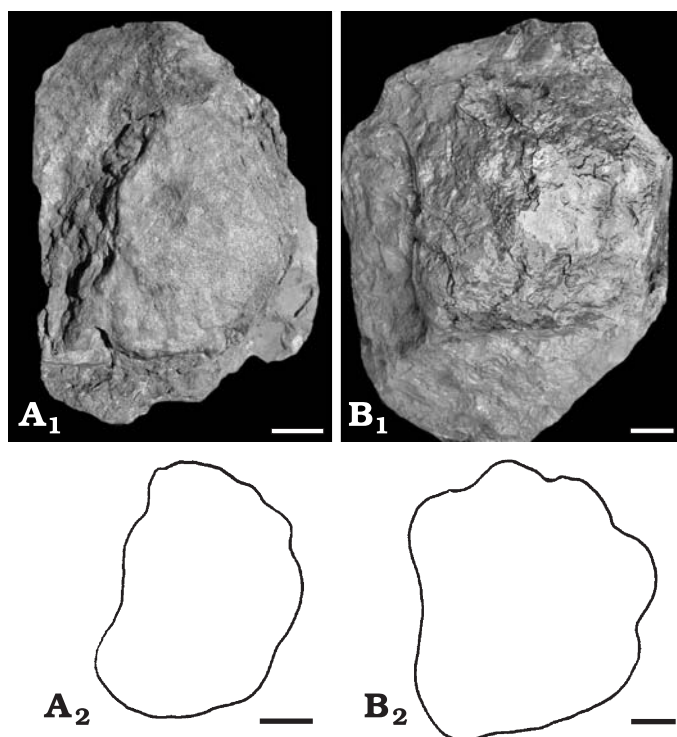
Fig. 6. ?Saupodomorph tracks indet. A. Specimen from the Czerwone Źlebki found in 2004, Tomanová Formation (?late Norian–Rhaetian), Poland. B. Specimen from the Červený Ůplaz found in 2007, Tomanová Formation (?late Norian–Rhaetian), Slovakia. Both specimens left in field. Photographs (A 1 , B 1 ) and drawings (A 2 , B 2 ). Scale bars 5 cm.
