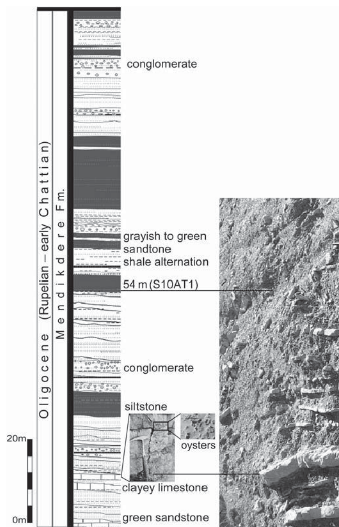
Fig. 2. The Kurucan section and sample location.
