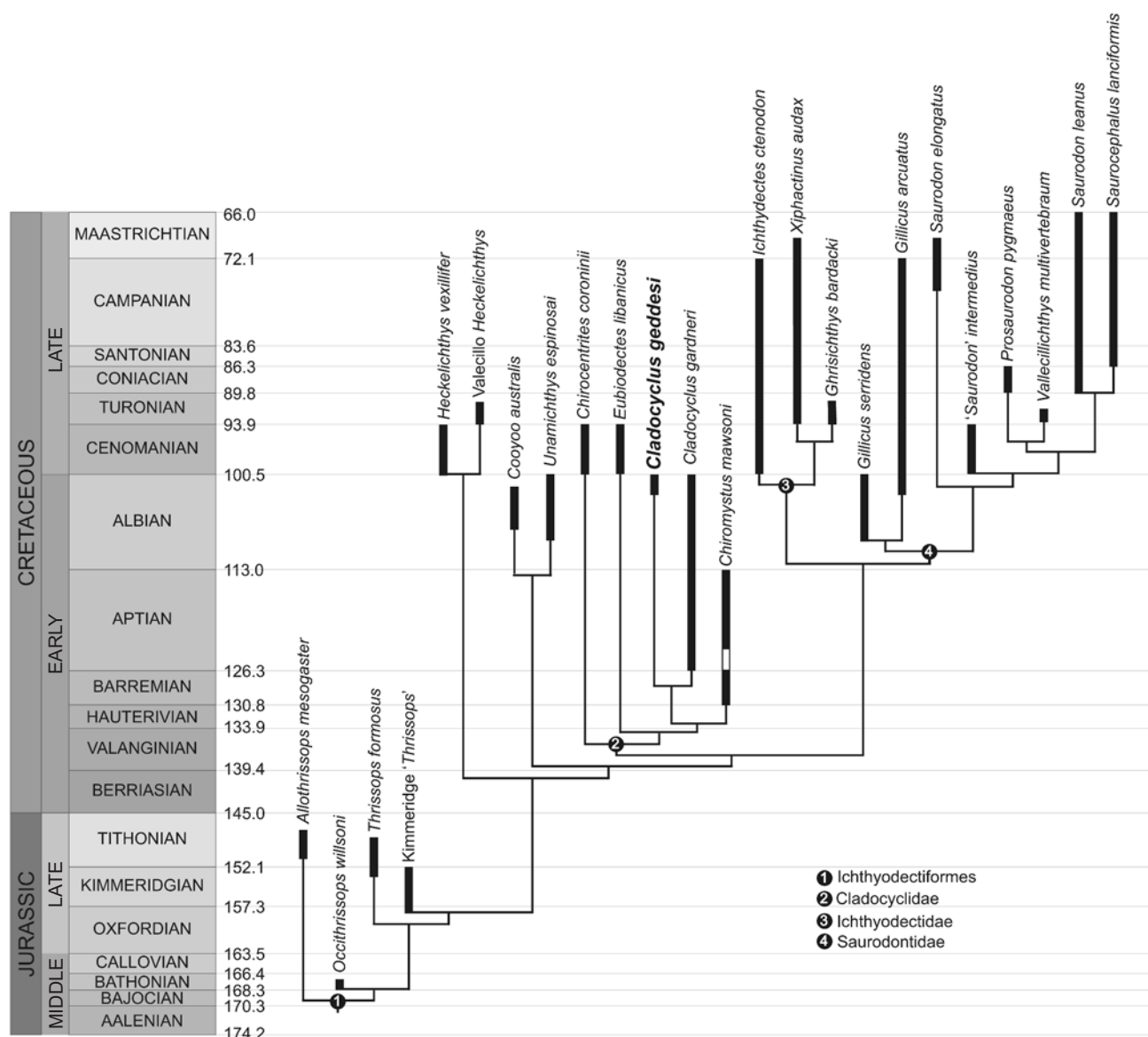
Fig. 8. Phylogenetic relationships of Cladocycclus geddesi sp. nov. (QM F44329). Stratigraphically calibrated strict consensus of 3 most-parsimonious trees (length 223, CI 0.45, RI, 0.67) analysed using T.N.T. 1.1 (Goloboff et al. 2003), with a heuristic search (1000 replicates in “Traditional search” with TBR branch swapping). See Appendix 1 for new character descriptions, taxon-character matrix, and a list of character state transformation for each taxon. Age ranges correspond to those provided in Cavin et al. (2013).
