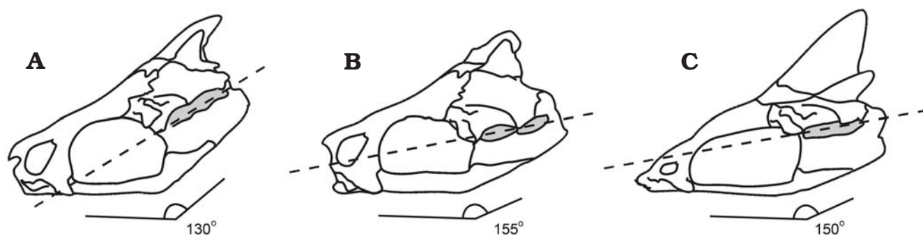
Fig. 6. Projection of the hyomandibular facet and angle of the parasphenoid in three ichthyodectiform fishes. A. Cladocycclus gardneri Agassiz, 1841 (based on AMNH 19129). B. Aidachar pankowskii (Forey and Cavin, 2007) (after Forey and Cavin 2007: fig. 4). C. Ichthyodectes ctenodon Cope, 1871 (after Badack 1965: 14). Also, note differences in proportions of the skull in these ichthyodectiforms. QM F44329 ( Cladocycclus geddesi sp. nov.) has the same angle of the parasphenoid as Cladocycclus gardneri .
