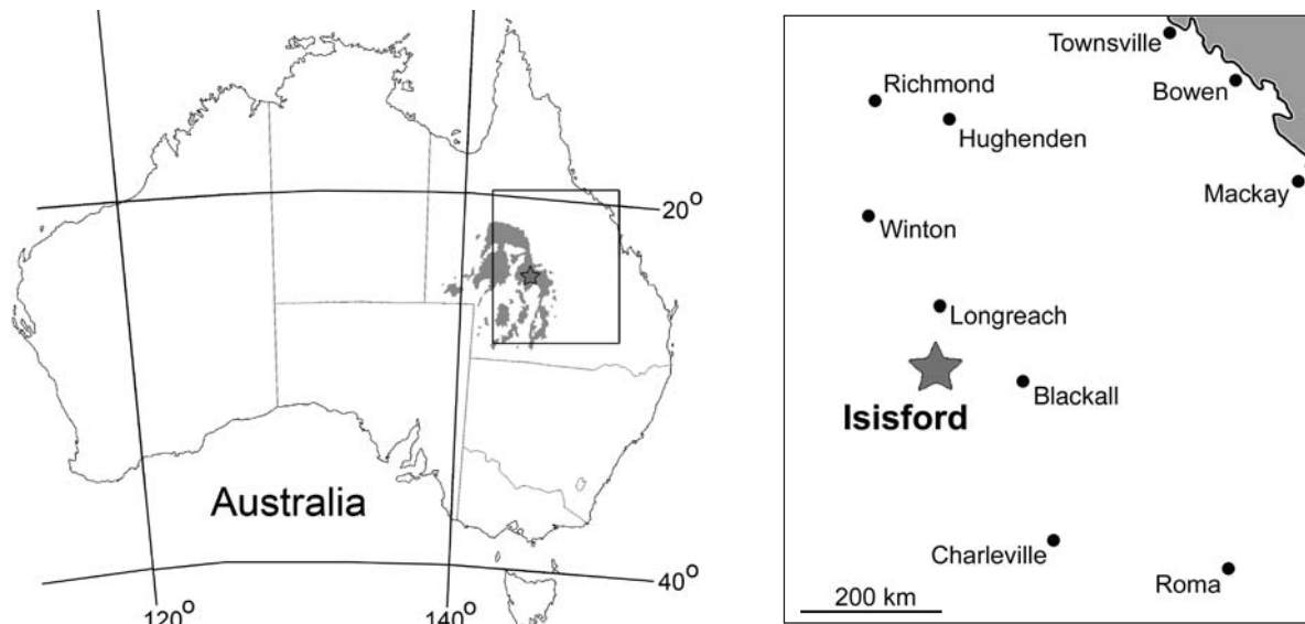
Fig. 1. Map showing the discovery site of Cladocycclus geddesi sp. nov. (QM F44329) near the town of Isisford, central-western Queensland, Australia. Gray area indicates the extent of the upper Albian–lower Turonian Winton Formation.
