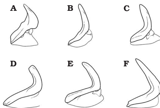
Fig. 7. Outlines of various ichthyodectiform pectoral girdle (cleithrum, coracoid, and scapular) arrangements in lateral external view. A. Alloth-rissops mesogaster (Agassiz, 1843) (redrawn from Patterson and Rosen 1977: fig. 10). B. Thrissops formosus Agassiz, 1833 (redrawn from Taverne 1977: fig. 5). C. Unamichthys espinosai Alvarado-Ortega, 2004 (IGM 8373). D. Cladocycclus geddesi sp. nov. (QM F44329). E. Cladocycclus gardneri Agassiz, 1841 (AMNH 11877). F. Vallecillichthys multivertebra-tum Blanco and Cavin, 2003 (redrawn from Blanco-Piñón 2003: fig. 9.2).
