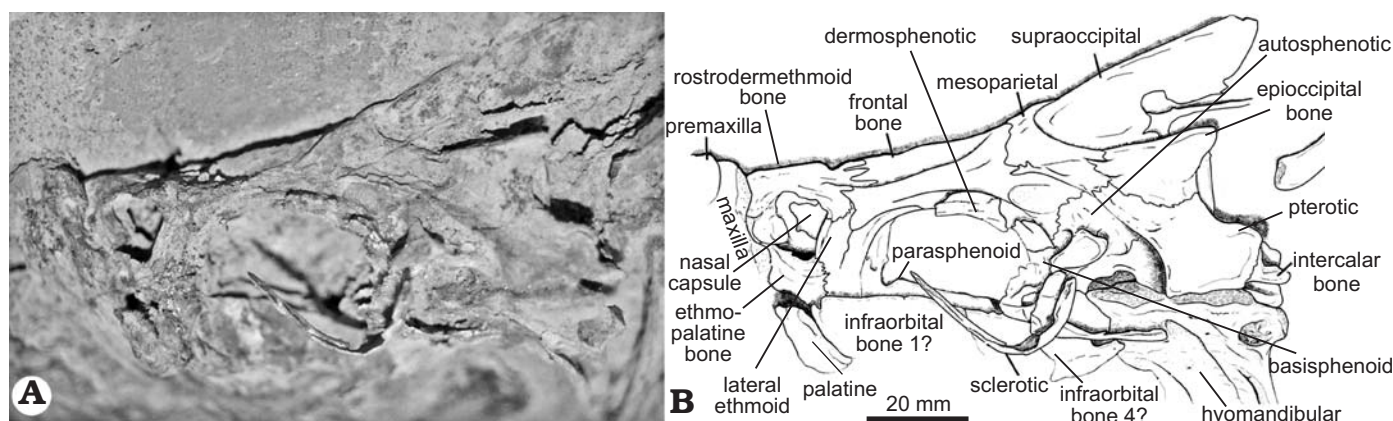
Fig. 4. Ichthyodectiform fish Cladocycclus geddesi sp. nov. (QM F44329) from near Isisford, central-western Queensland, Australia; Lower Cretaceous (upper Albian) strata of the Winton Formation, braincase in dorsolateral view. Photograph (A) and interpretive drawing (B).
