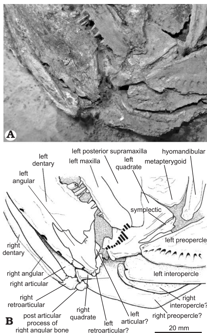
Fig. 5. Ichthyodectiform fish Cladocycus geddesi sp. nov. (QM F44329) from near Isisford, central-western Queensland, Australia; Lower Cretaceous (upper Albian) strata of the Winton Formation, area of articulation for the lower jaw. Photograph (A) and interpretive drawing (B). Hatched area indicates broken bone.
