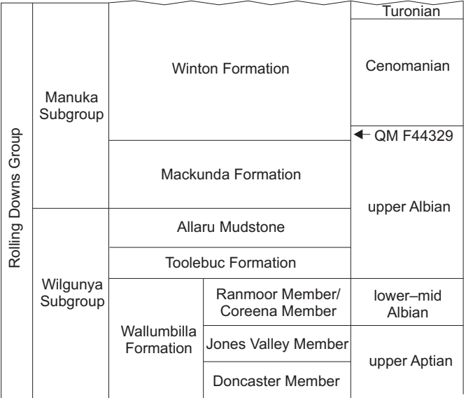
Fig. 2. Stratigraphy of the Eromanga Basin, western Queensland, after Gray et al. (2002) and Tucker et al. (2013). Cladocycclus geddesi sp. nov. (QM F44329) comes from the lower part of the Winton Formation, and is upper Albian in age.
