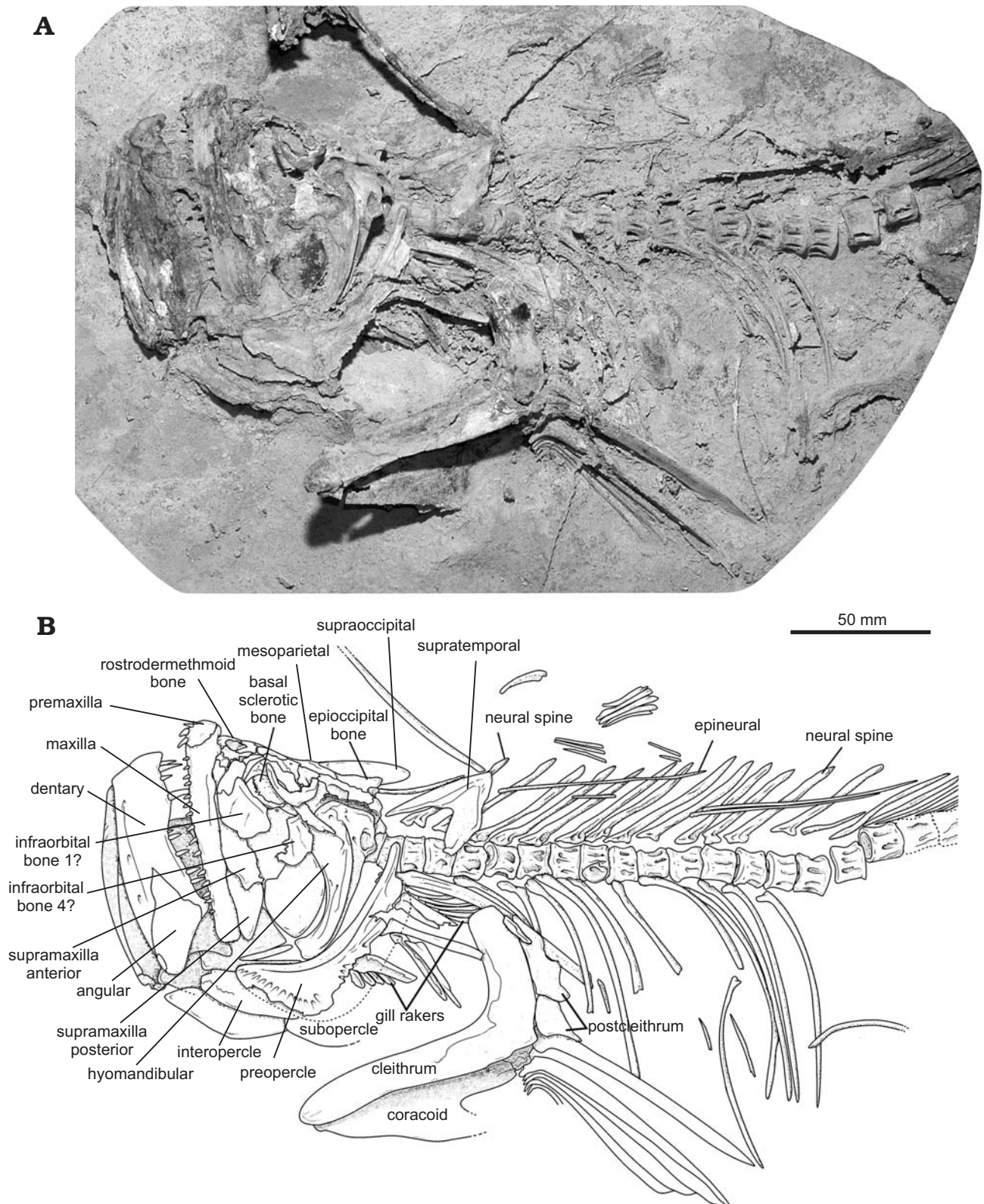
Fig. 3. Ichthyodectiform fish Cladocyclus geddesi sp. nov. (QM F44329) from near Isisford, central-western Queensland, Australia; Lower Cretaceous (upper Albian) strata of the Winton Formation, in lateral view. Photograph (A) and interpretive drawing (B).
