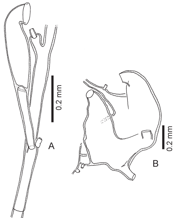
Fig. 10. Zygophylax sibogae MHNG-INVE-69633. (A) Part of hydrocladium with one hydrotheca. Note the presence of a small nematotheca on the apophysis. (B) Gonothecha, note irregular shape.
