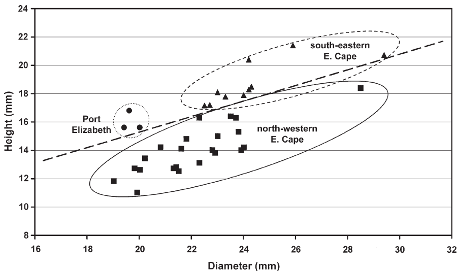
Fig. 60. Afrophytida knysnaensis (Pfeiffer, 1846), plot of height/diameter measurements, showing differing shell proportions in different populations. The diagonal dashed line corresponds to the line drawn between St Francis Bay and Molteno in the distribution map (Fig. 59).
