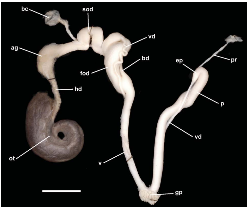
Fig. 74. Capitina calcicola sp. n., reproductive tract (paratype, NMSA W5670/T2265), scale bar = 5.0 mm.
