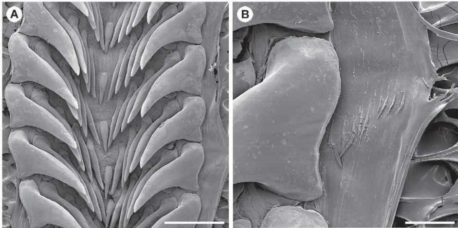
Fig. 28. Natalina cafra natalensis subsp. n., radula, Karkloof Forest (NMSA V8415): (A) rachidian and lateral teeth, scale bar = 1.0 mm; (B) vestigial marginal teeth, scale bar = 250 µm.
