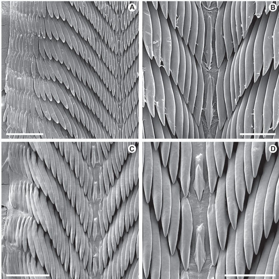
Fig. 73. Capitina species, radula: (A, B) Capitina schaerfiae (Pfeiffer, 1861), Oubos (NMSA W5672), scale bars = 300 µm and 100 µm; (C, D) Capitina calcicola sp. n., Cape Agulhas (paratype, NMSA W3360/T2270), scale bars = 200 µm and 100 µm.
