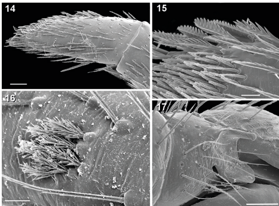
Figs 14–17. Dioreis similis sp. n. SEM views; female, Mkomazi (MRAC 215697): (14) female palp, dorsal view; (15) detail of previous showing modified pectinated setae and truncated chemosensitive setae; male paratype, Mkomazi (MRAC 215731): (16) femoral organ leg 2, retrolateral view; (17) male palp, tibia, showing RTA. Scale bars: (14) = 100 µm, (15) = 200 µm, (16) = 20 µm, (17) = 50 µm.
