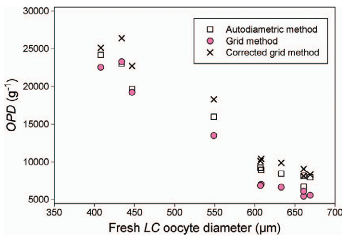
FIGURE 4. Oocyte packing density (OPD; number of oocytes/g of ovary) for developing oocytes of Atlantic cod in relation to fresh leading cohort (LC) oocyte diameter estimated by the grid method (Table 3), the corrected grid method (see Results), and the autodiametric method. Samples with LC diameters less than 500 \mu\text{m} contained developing oocytes characterized as cortical alveolar, early vitellogenic, and late vitellogenic oocytes, while for LC diameters greater than 500 \mu\text{m} the only developing type was late vitellogenic oocytes.
