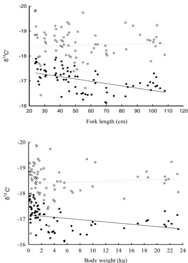
FIGURE 3. Relationship between \delta^{13}C' values and both (a) fork length and (b) body weight of Yellowfin Tuna. White muscle is represented by the a solid line and filled circles, and liver is represented by a dashed line and open circles. In panel (a) \delta^{13}C' = -17.546 - 0.0093FL for white muscle and \delta^{13}C' = -18.367 + 0.0012FL for liver. In panel (b) \delta^{13}C' = -17.158 + 0.023BW for white muscle and \delta^{13}C' = -18.397 + 0.0069BW for liver.
