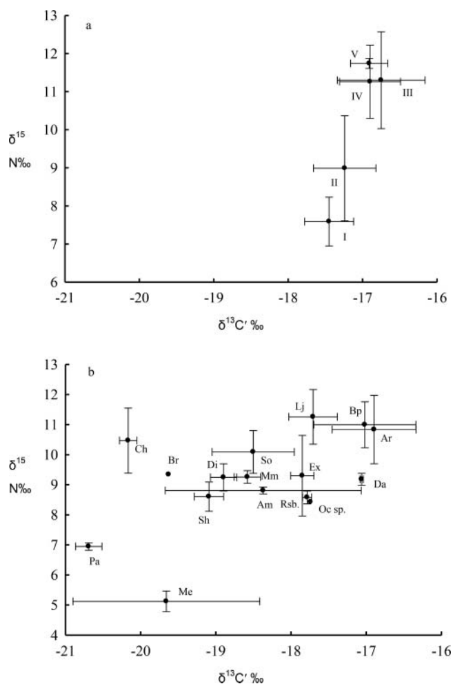
FIGURE 4. Mean \delta^{13}C' and \delta^{15}N values of (a) the white muscle of Yellowfin Tuna size-classes I–V and (b) prey species. R sp. = Rastrelliger sp.; Ar = Auxis rochei ; Lj = Lestrolepis japonica ; Oc sp. = Octopus sp.; Ex = Exocoetidae; Am = Amphipoda; Ch = larval Chaetodontidae; Sh = postlarval shrimps; Bp = Benthoosema pterotum ; So = Sthenoteuthis oualaniensis ; Pa = Faughina spp.; Me = larval crabs; Br = Brama sp. Vertical and horizontal bars represent SD values.
