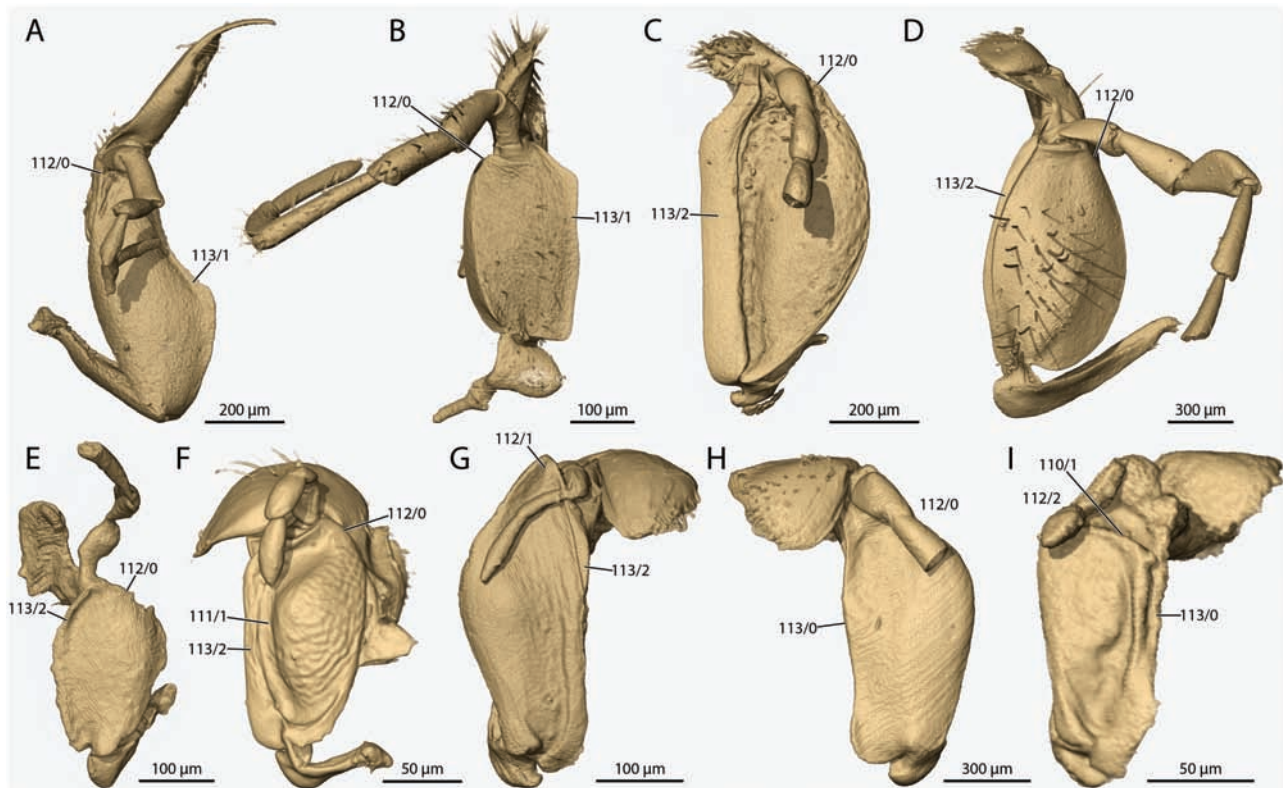
Char. 110–113. 3D reconstructions of the maxilla in external view onto the stiptal sclerite, A: Parischnogaster sp., B: Methocha sp., C: Ampulex sp., D: Sceliphron caementarium , E: † Gerontoformica gracilis , F: Protanilla lini , G: Brachyponera luteipes , H: Formica rufa , I: Wasmannia affinis . Char. 110: transverse stiptal groove, (0): absent, (1): present. Char. 111: longitudinal stiptal groove, (0): absent, (1): present. Char. 112: Shape of distal stiptal margin laterad palpus, (0): flat, (1): acute process, (2): laterally extended shoulder. Char. 113: Medial stiptal flange, relative to stiptal surface, (0): not raised, (1): raised in gentle curve, (2): raised in distinct step.
