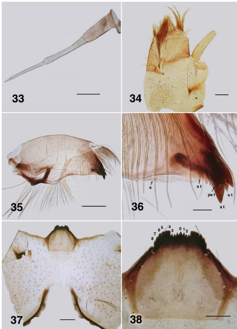
Figs. 33–38. Ectemnodoides umbratorum last instar larva (Grampians). (33) Antenna. Scale bar = 0.05 mm. (34) Maxilla. Scale bar = 0.05 mm. (35) Mandible. Scale bar = 0.1 mm. (36) Mandible apex. Abbreviations: a t – apical tooth; o t – outer teeth; sub t – subapical teeth; s – serrations and sensillum; s t – spinous teeth. Scale bar = 0.02 mm. (37) Postgenal cleft. Scale bar = 0.1 mm. (38) Hypostoma. Numbers indicate teeth. Scale bar = 0.05 mm.
