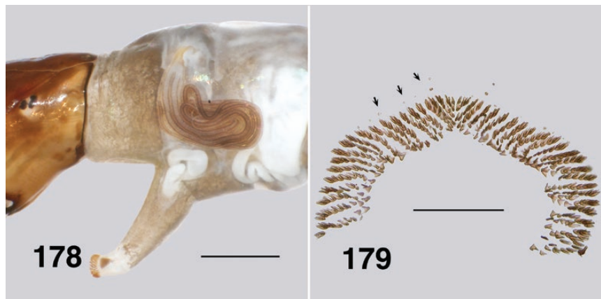
Figs. 178–179. Ectemnoidea princeae larva. (178) Pharate pupal gill. Scale bar = 0.5 mm. (179) Circllet of hooks. Note absence of anal sclerite. Arrows indicate campaniform sensilla. Scale bar = 0.2 mm.
