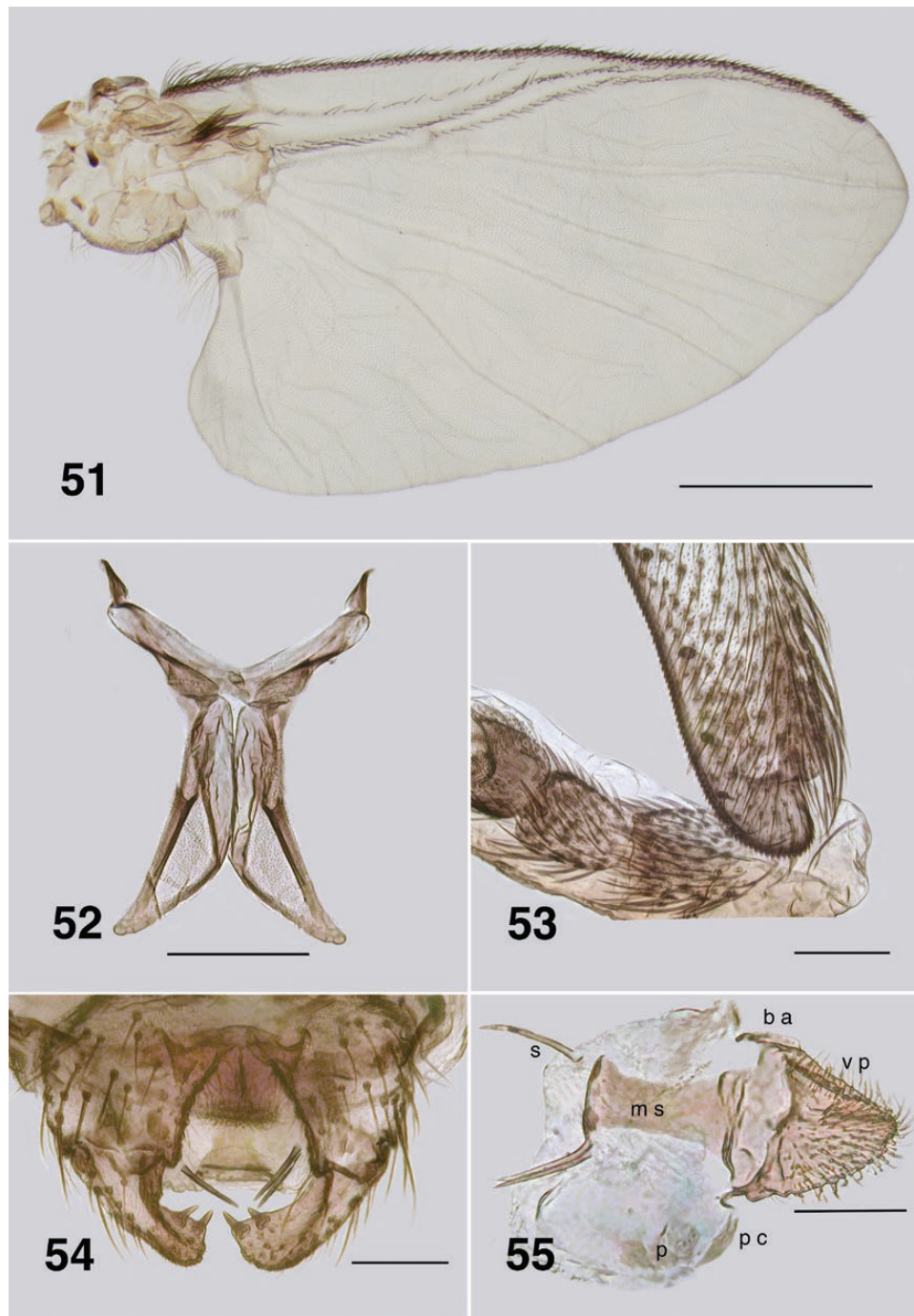
Figs. 51–55. Ectemnooides faecofilus male adult. (51) Wing. Paratype. Pharate. Scale bar = 0.5 mm. (52) Metathoracic furcasternum. Scale bar = 0.1 mm (53) Hind basitarsus and tarsomere II. Partially encased in pupal exuviae. Scale bar = 0.05 mm. (54) Ventral view of genitalia. Scale bar = 0.05 mm. (55) Slide mount of genitalia. b a – basal arm; m s – median sclerite; p – paramere; p c – paramere connector; s – spines; v p – ventral plate. The ventral plate is flipped 90 degrees to the right. Scale bar = 0.05 mm.
