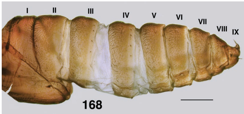
Figs. 168. Ectemnoidea princeae pupal abdomen showing armature. Scale bar = 0.5 mm.
