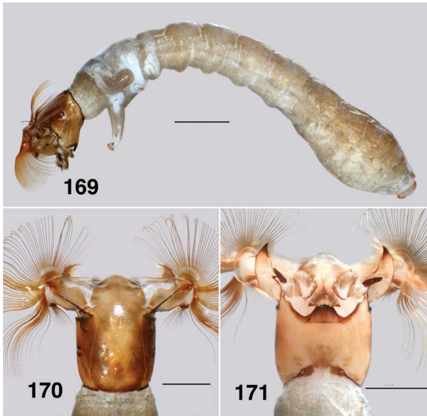
Figs. 169–171. Ectemnoidea princeae last instar larva. (169) Habitus. Scale bar = 1.0 mm. (170) Dorsal view of the head. Scale bar = 0.5 mm. (171) Ventral view of the head. Scale bar = 0.5 mm.
