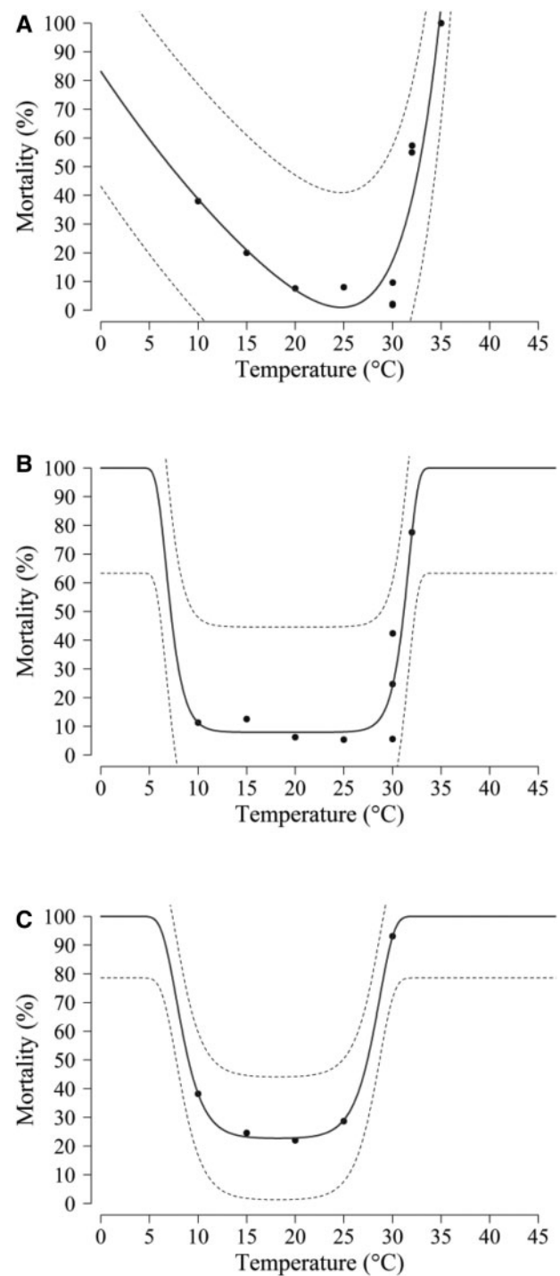
Fig. 3. Temperature-dependent mortality rates of immature life stages of L. huidobrensis : egg (A), larvae (B), and pupae (C). Fitted curves: Gompertz-Makeham model (A), Wang 2 model (B, C). Dashed lines above and below represent the upper and lower 95% confidence.
