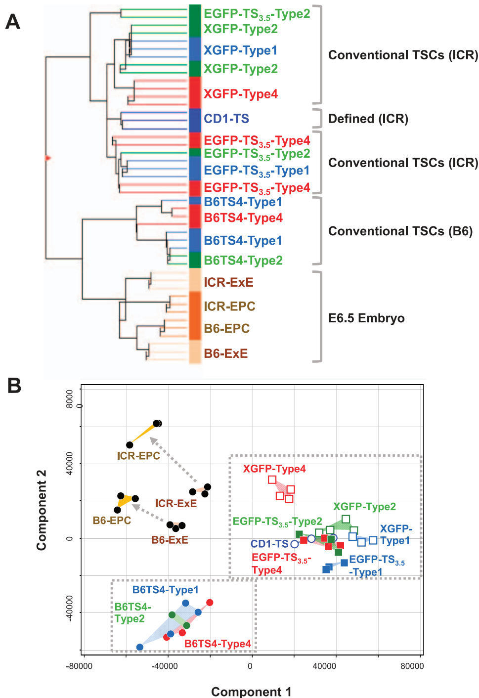
FIG. 5. Microarray analysis for global gene expression profiles in TSC colonies and in vivo-derived extraembryonic tissues. A ) Hierarchical clustering analysis. Trophoblast stem cell samples were clustered by their genetic background (B6 vs. ICR strain) rather than by their colony type. B ) Principal component analysis. The TSC samples were grouped by their genetic backgrounds. For the numbers of samples, see Table 1.
