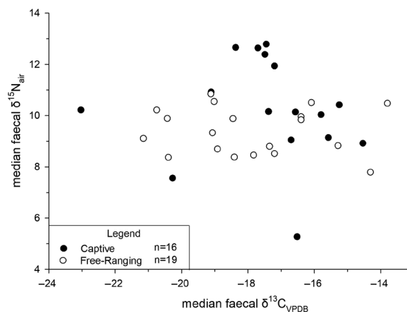
Figure 3. Median faecal \delta^{15}\text{N} values plotted against median faecal \delta^{13}\text{C} values obtained for each African wild dog (AWD) monitored.
