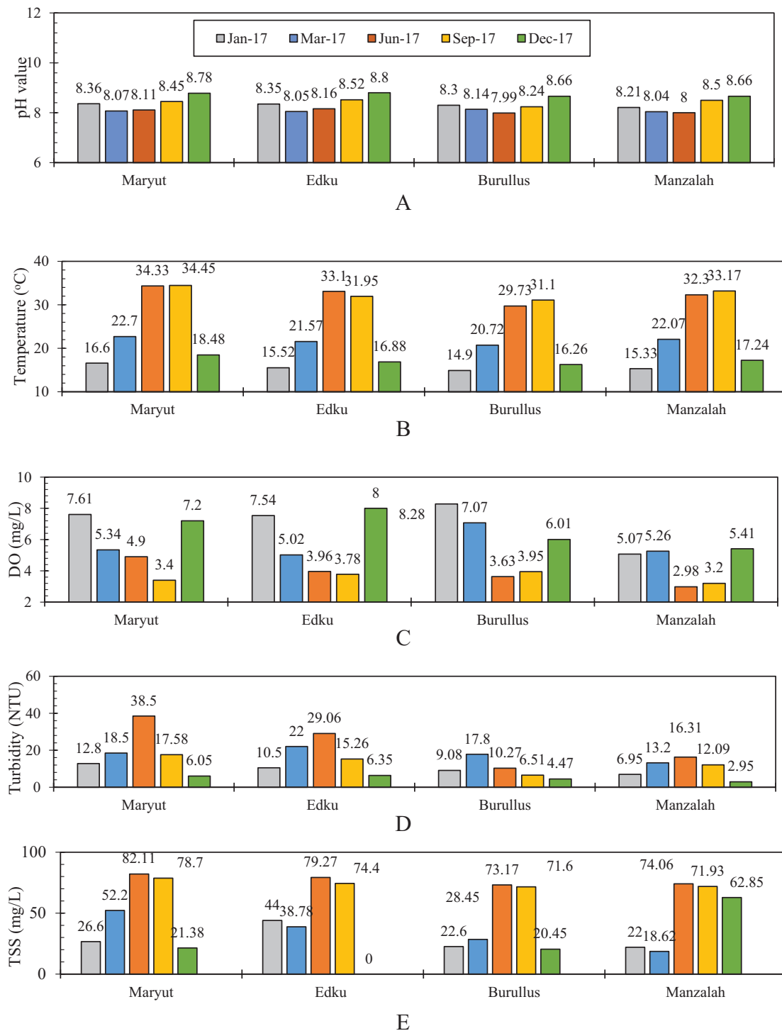
Figure 3. Water physical properties of Nile Delta lagoons during year 2017 where: (A) pH, (B) temperature, (C) dissolved oxygen (DO), (D) turbidity and (E) total suspended solids (TSS).
