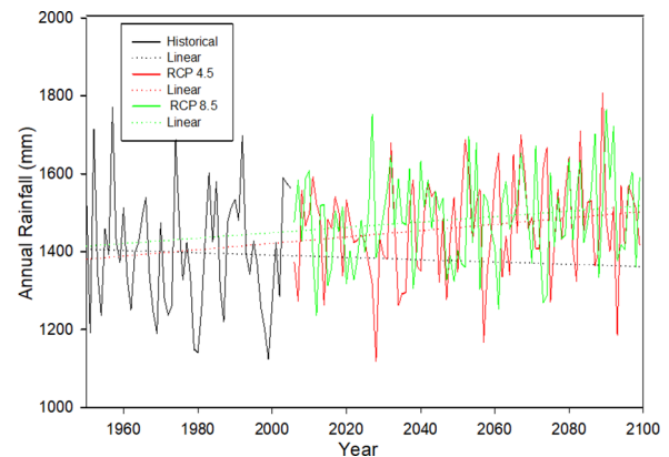
Figure 5. Annual precipitation trend analysis with averaged model data. Historical timeline: 1950-2005 and future timeline: 2006-2099 for both RCP8.5 and RCP4.5 scenarios. RCP indicates Representative Concentration Pathway.
