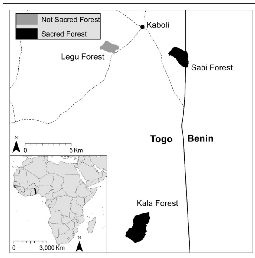
Figure 1. Map of the Legu, Sabi, and Kala community forests. Dotted lines represent major roads, and solid lines represent the Togo–Benin border. Inset in bottom left corner shows the location of Togo (in black) in Africa.
