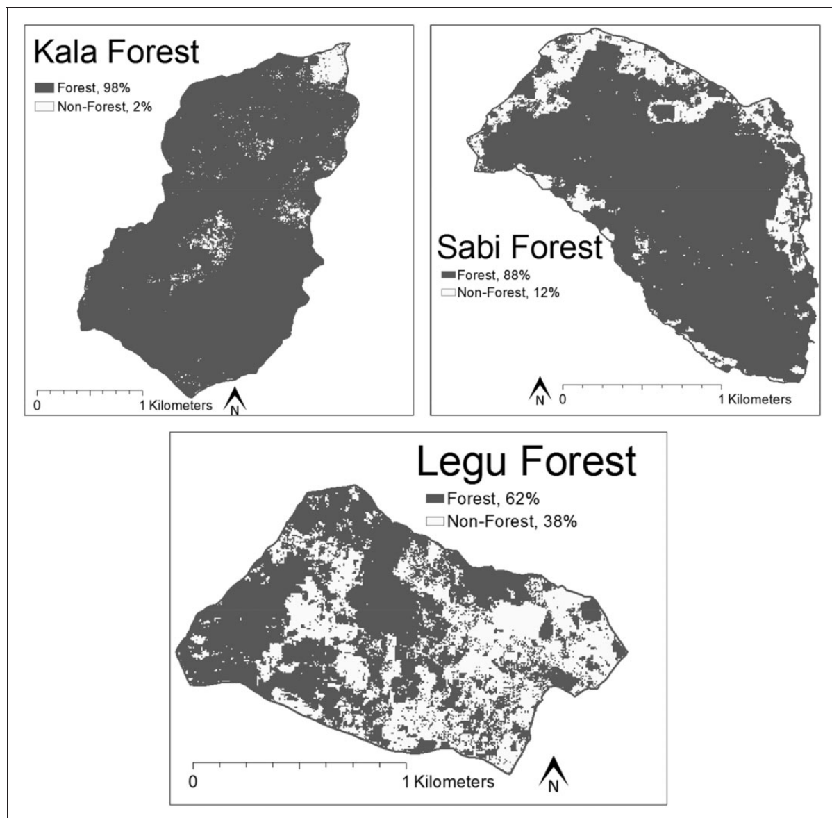
Figure 3. Land cover maps of each of the three forests considered in this study. The Sabi and Kala Forests are sacred forests while the Legu Forest does not contain a sacred site.
