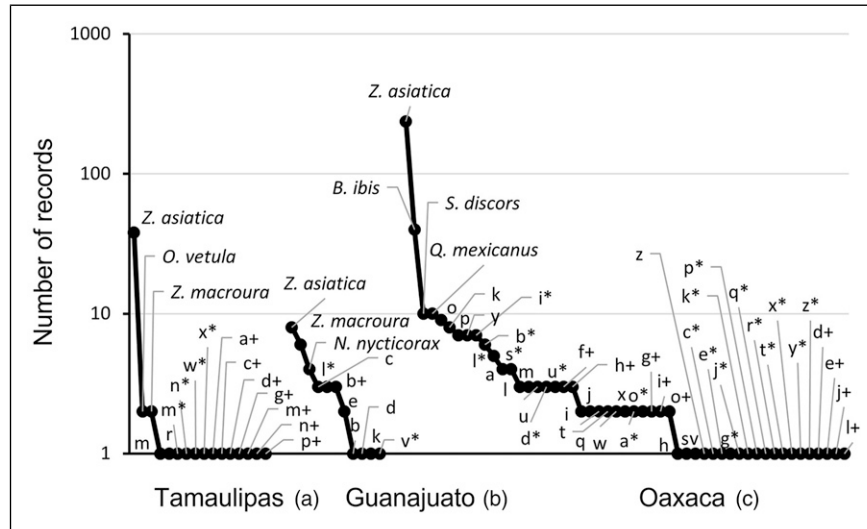
Figure 3. Rank-abundance plots for species with carcasses recorded in the sampled sites of Tamaulipas (a), Guanajuato (b) and Oaxaca (c), Mexico. The species codes are included in Table 1. a= Dendrocygna autumnalis , b= Mareca strepera , c= Mareca americana , d= Anas platyrhynchos , e= Anas diazi , f= Spatula discors , g= Ortalis vetula , h= Ortalis poliocephala , i= Colinus virginianus , j= Columbina inca , k= Columbina passerina , l= Columbina spp., m= Leptotila verreauxi , n= Zenaida asiatica , o= Zenaida macroura , p= Crotophaga sulcirostris , q= Morococcyx erythropygus , r= Geococcyx californianus , s= Chordeiles sp., t= Chordeiles acutipennis , u= Nyctidromus albicollis , v= Porzana carolina , w= Porphyrio martinicus , x= Aramus guaranauna , y= Burhinus bistriatus , z= Gallinago delicata , a*= Leucophaeus atricilla , b*= Leucophaeus pipixcan , c*= Ardea herodias , d*= Ardea alba , e*= Egretta caerulea , f*= Bubulcus ibis , g*= Butorides virescens , h*= Nycticorax nycticorax , i= Eudocimus albus , j*= Platalea ajaja , k*= Coragyps atratus , l*= Cathartes aura , m*= Tyto alba , n*= Bubo virginianus , o*= Caracara cheriway , p*= Falco sparverius , q*= Eupsittula canicularis , r*= Pitangus sulphuratus , s*= Tyrannus melancholicus , t*= Tyrannus verticalis , u*= Tyrannus forficatus , v*= Corvus corax , w*= Poliophtila caerulea , x*= Turdus grayi , y*= Mimus gilvus , z*= Mimus polyglottos , a+= Arremonops rufivirgatus , b+= Spizella passerina , c+= Junco hyemalis , d+= Melospiza lincolni , e+= Sturnella magna , f+= Icterus spp., g+= Icterus spurius , h+= Icterus pustulatus , i+= Icterus gularis , j+= Molothrus aeneus , k+= Quiscalus mexicanus , l+= Seiurus aurocapilla , m+= Geothlypis philadelphia , n+= Setophaga sp., o+= Setophaga petechia , p+= Cardinalis cardinalis .
