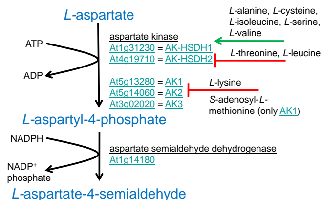
Figure 3. Biosynthesis of L -aspartate-4-semialdehyde from L -aspartate. These two enzymatic steps that are common to all branches of the aspartate-derived amino acid pathway. Known allosteric regulation is shown, activation with a green arrow and inhibition with a red bar.
