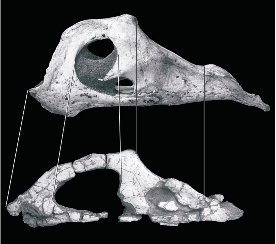
Fig. 13. The holotype mandibles of Citipati osmolskiae IGM 100/978 (top) and Oviraptor philoceratops AMNH 6517 (bottom) in left lateral view (not to scale). The Oviraptor mandible has been digitally compressed to minimize the separation at two breaks in the dentary. Lines are drawn between topologically comparable points on the two mandibles to illustrate the proportionately greater length of the anterior part of the O. philoceratops mandible.
