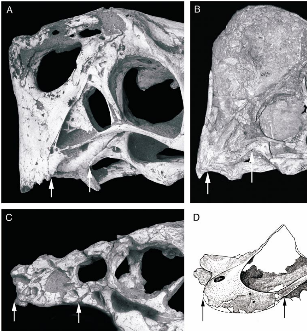
Fig. 12. Rostral regions (not to scale) of (A) the holotype of Citipati osmolskae IGM 100/978, (B) the holotype of "Oviraptor" mongoliensis (IGM 100/32) (reversed), (C) the holotype of Oviraptor philoceratops AMNH 6517, and (D) a referred specimen of the caenagnathid Chirostenotes pergracilis (ROM 43250) (from Sues, 1997). The maxilla of O. philoceratops is relatively longer than in the oviraptorids (B and C) but shorter than in the caenagnathid (D), which represents the plesiomorphic condition for oviraptorosauroids. Arrows indicate premaxilla-maxilla contact anteriorly and palatine-maxilla contact posteriorly. Abbreviations in appendix 1.
