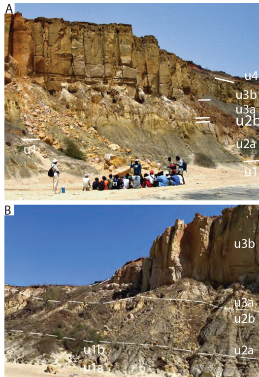
FIGURE 4. The four units visible at the Cap de Naze Cliff locality with the end Campanian Paki Formation and the Late Maastrichtian Cap de Naze Formation cropping out under a Pliocene capping. A , units 1–4 (figure modified from Cuny et al., 2012: fig. 2) and B , units 1–3.
