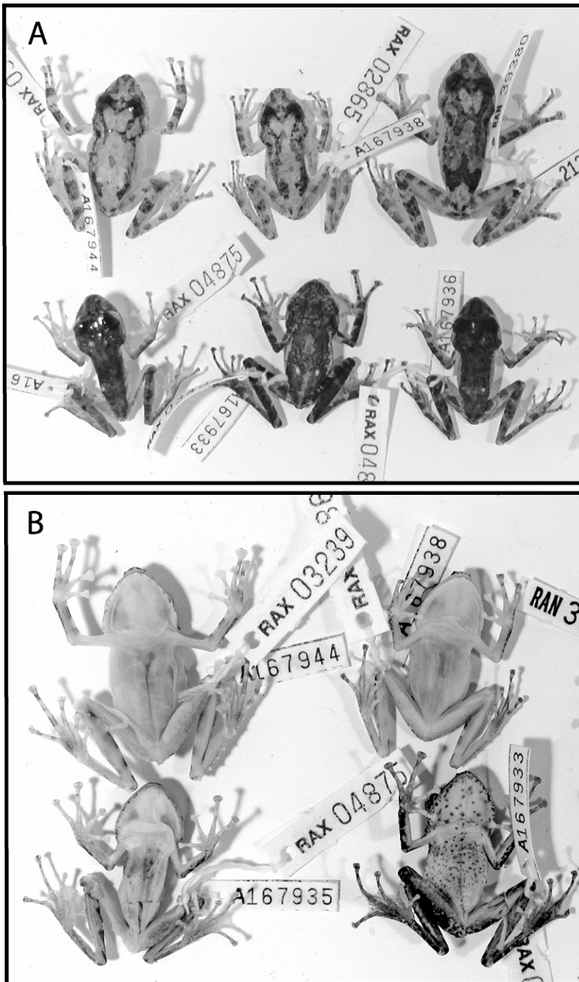
Fig. 3. Spinomantis massorum and S. tavaratra , new species. A. Dorsal views of S. massorum (above, left to right): AMNH A167944, 167938, UMMZ 212359; and S. tavaratra , new species (below, left to right): AMNH A167935, 167933, 167936. B. Ventral views of S. massorum (above, left to right): AMNH A167944, 167938; and S. tavaratra , new species (below, left to right): AMNH A167935, 167933.
