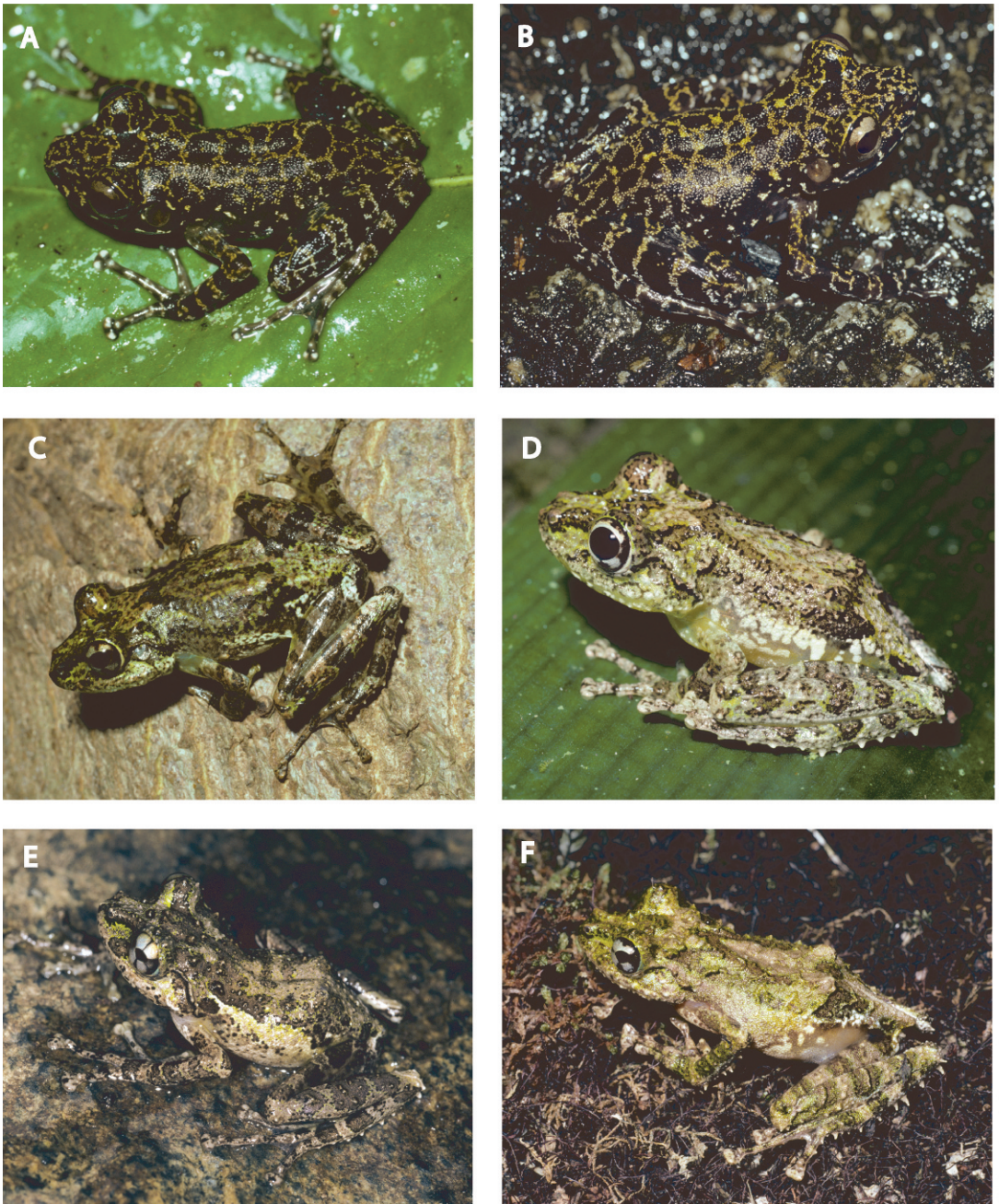
Fig. 1. Photos of selected live Spinomantis species. A. Spinomantis brunae , UMMZ 198405, Ampamakiesiny Pass (photo: C.J. Raxworthy). B. S. brunae , UMMZ 198407, Ampamakiesiny Pass (photo: C.J. Raxworthy). C. S. massorum , UMMZ 212362, Antsahabe River, Manongarivo Special Reserve (photo: C.J. Raxworthy). D. S. massorum , AMNH A167941, Ramena River, Tsaratanana Strict Nature Reserve (photo: C.J. Raxworthy). E. S. tavaratra , new species, AMNH A167937, Sorata Mountain (photo: C.J. Raxworthy). F. S. aglavei , UMMZ 212374, Andringitra Strict Nature Reserve (photo: C.J. Raxworthy).
