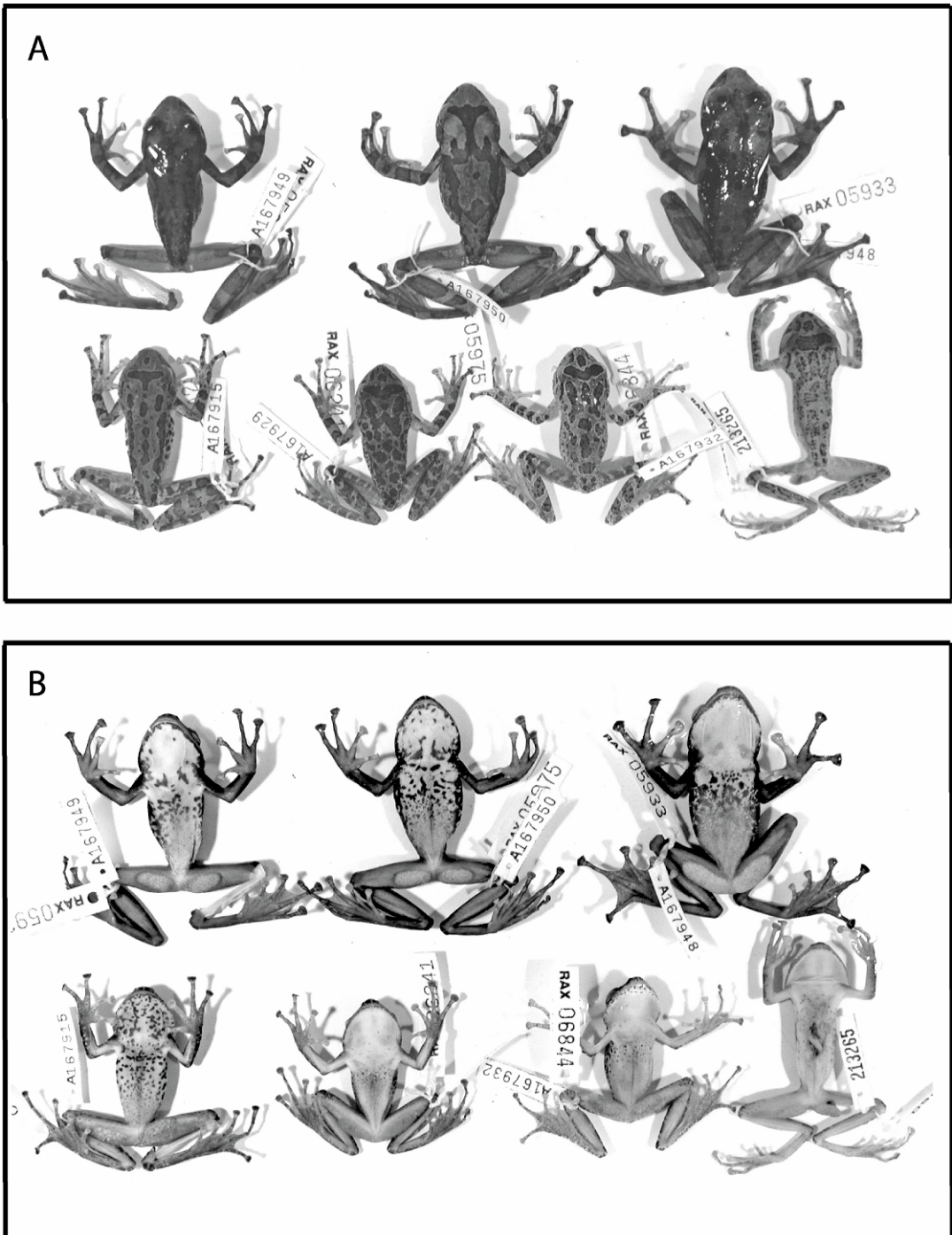
Fig. 4. Spinomantis nussbaumi , new species, and S. peraccae . A. Dorsal views of S. nussbaumi , new species (above, left to right): AMNH 167949, 167950, 167948; and S. peraccae (below, left to right): AMNH 167915, 167929, 167932, UMMZ 213265. B. Ventral views of S. nussbaumi , new species (above, left to right): AMNH 167949, 167950, 167948; and S. peraccae (below, left to right): AMNH 167915, 167929, 167932, UMMZ 213265.
