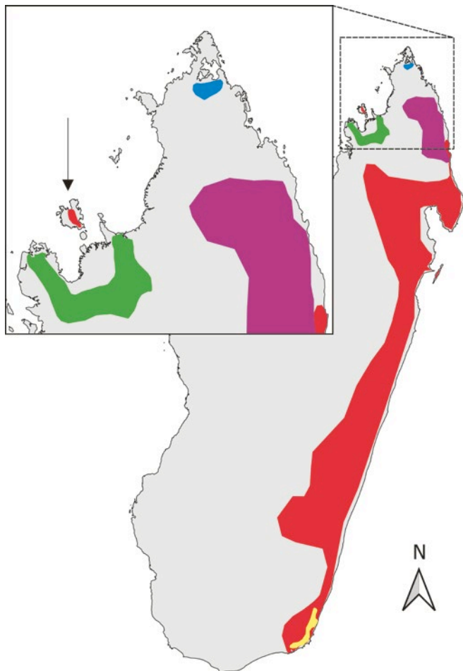
Fig. 1. – Map showing the approximate distribution ranges for Dalbergia Group II species treated in the text. From north to south: D. antsirananae Phillipson, Cramer & N. Wilding (blue); D. viguieri Bosser & R. Rabev. (purple); D. manongarivensis Bosser & R. Rabev. (green); D. madagascariensis Vatke (red; note small subpopulation on Nosy Be, indicated by an arrow); D. delphinensis Bosser & R. Rabev. (yellow).
