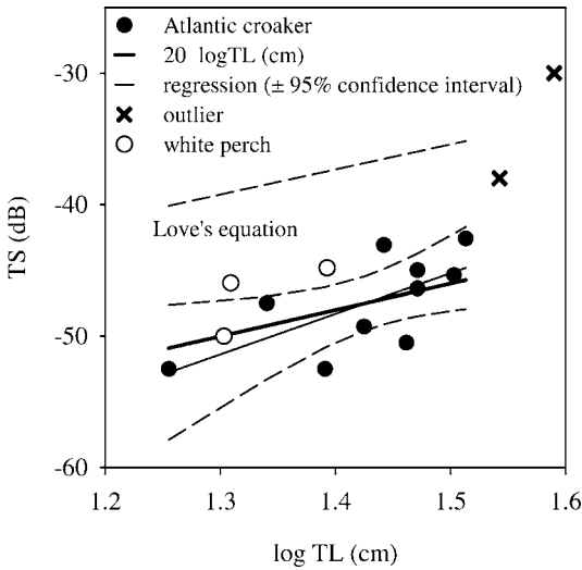
FIGURE 6.—Comparison of three equations depicting the relationship between dorsal aspect total length (TL, cm) and target strength (TS; decibels [dB]) of Atlantic croakers (black circles; \times = outliers; CI = confidence interval): (1) least-squares regression ( TS = a \cdot \log_{10}[TL] + b , where b = intercept and a = slope; thin solid line), (2) regression assuming quadratic dependence ( TS = 20 \cdot \log_{10}[TL] + b ; heavy solid line), and (3) Love's (1971) equation ( TS = 19.1 \cdot \log_{10}[TL] + 0.9 \cdot \log_{10}[\text{frequency}] - 62 ; straight dashed line). White perch data (open circles) are also presented but were not subject to regression analysis.
