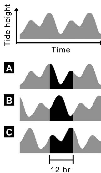
FIGURE 1. (Top) A mixed semi-diurnal tide (grey) results in 2 low tides per 24-hour period, each of unequal tide height, which differentially impacts shallow-water availability. The tidal signature (grey) shifts about 1 hr daily, resulting in daily (A–C), daytime (black, 12-hr) differences in low tide height. Time-shifts in the tidal pattern are more likely to affect daytime-only foragers such as the Little Blue Heron. By contrast, time-shifts in the tidal pattern should not affect species, such as the Great White Heron, that have the behavioral flexibility to access low tides during the day and night.
