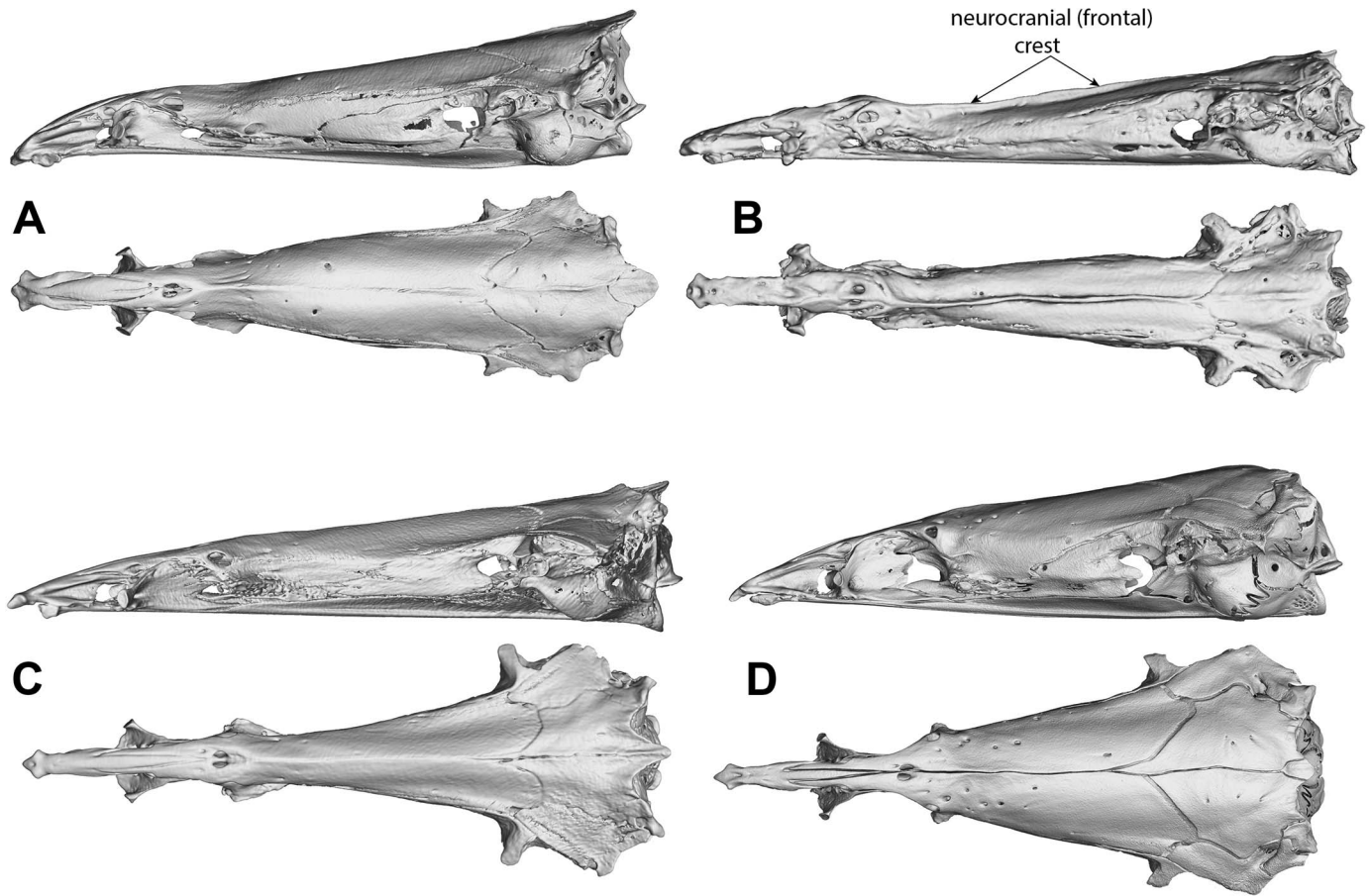
Fig. 9. Comparative osteology of the neurocranium. Neurocrania in lateral and dorsal views of: (A) Ophisternon berlini , new species (paratype, AMNH 281171, 162 mm TL), (B) Ophisternon infernale (AMNH 272953, 240 mm TL), (C) Ophisternon aenigmaticum (holotype, AMNH 32410, 358 mm TL), and (D) Ophisternon aenigmaticum (paratype, AMNH 32408, 154 mm TL). Not to scale.
