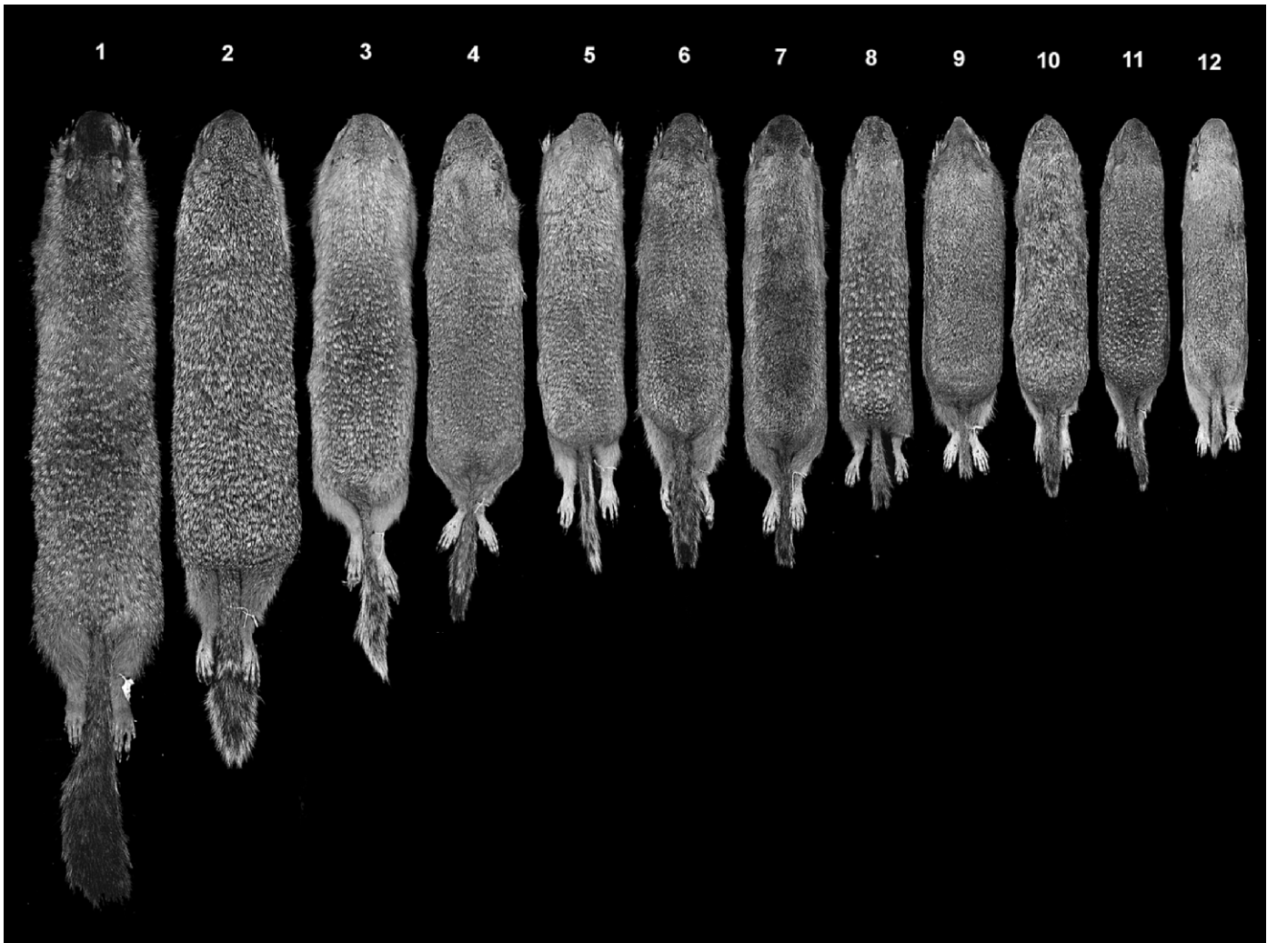
FIG. 16. —Representative skins (all adult females) of the species of Urocitellus , including the “big-eared ground squirrels” (1–7) and the “small-eared ground squirrels” (8–12): 1) U. parryii , USNM 128620, Yukon River, Alaska, United States; 2) U. columbianus , USNM 236182, Gifford, Washington, United States; 3) U. undulatus , USNM 175312, Altai Mountains, Siberia, Russia; 4) U. elegans , USNM 179821, Evanston, Wyoming, United States; 5) U. richardsonii , USNM 225873, Livingston, Montana, United States; 6) U. armatus , USNM 18830, Fort Bridger, Wyoming, United States; 7) U. beldingi , USNM 88285, McKinney, California, United States; 8) U. washingtoni , USNM 78578, Pendleton, Oregon, United States; 9) U. townsendii , USNM 235742, Ellensburg, Washington, United States; 10) U. mollis , USNM 201605, Payette, Idaho, United States; 11) U. brunneus , USNM 202410, Van Wyck, Idaho, United States; 12) U. canus , USNM 204835, Bend, Oregon, United States.
