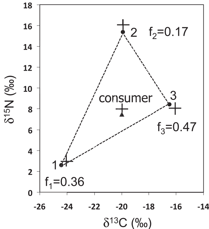
FIG. 3. —Illustration of the sensitivity of diet mixing model results to variability in isotope values of consumers and food sources. The error bars show the mean \pm 1 SE for the \delta^{13}\text{C} and \delta^{15}\text{N} isotope values for 3 food sources and a consumer as shown in Fig. 2. Alternative plausible values within these error ranges for the food sources (circles) and consumer (triangle) were used in a mixing model (note the offset from mean values), which resulted in different diet proportions (compare to Fig. 2, which used the mean values).
