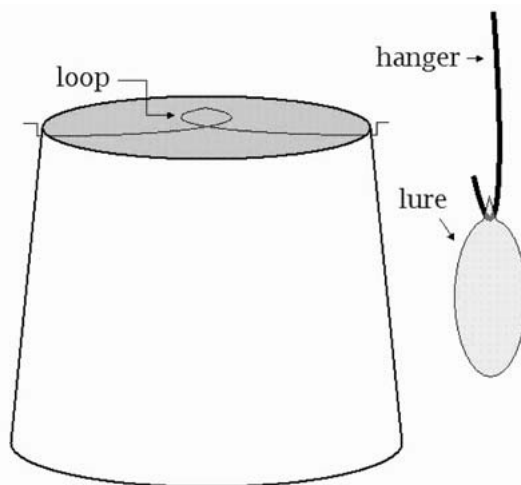
Fig. 1. Stand-alone sticky cylindrical trap for fruit flies constructed with yellow cardboard coated with Stickem Special (top diameter, 13.5 cm; bottom diameter, 16 cm; height, 13.5 cm). The lure and trap (at the loop in the wire) can be suspended separately from the trap hanger.
